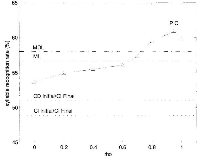
Fig. 3. PIC based decision tree construction is evaluated under different forgetting factors \rho . Syllable recognition rates of CI Initial/CI Final, CD Initial/CI Final, ML, and MDL based decision tree construction are compared.
