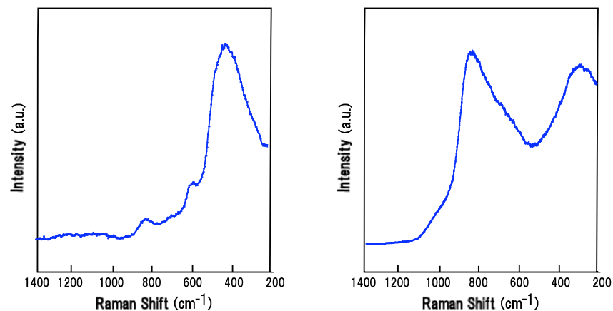
Fig. 3 Raman spectrum of optical fiber (left) and glass microsphere (right).
