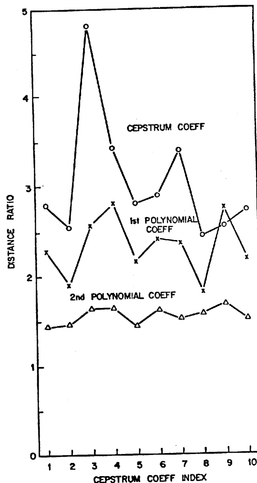
Fig. 2. Inter-speaker to intra-speaker distances for the first 10 utterances by 5 speakers from utterance set 1.
