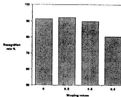
FIGURE 5 Recognition rates for frequency warped LSP distance measure
