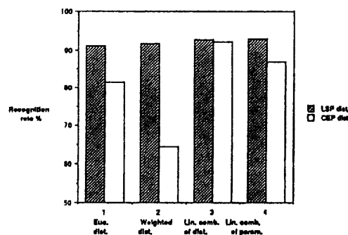
FIGURE 3 Recognition rates for various LSP distance measures
