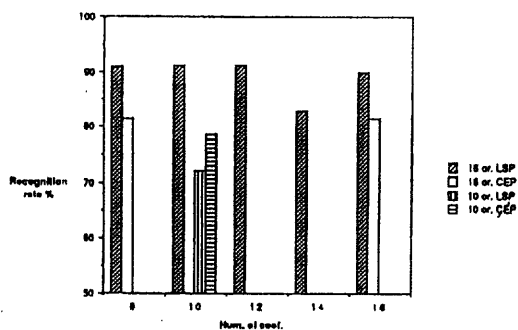
FIGURE 2 Recognition rates for LSP and cepstrum coefficients
