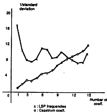
FIGURE 4 The relationship between the average inverse standard deviations of LSP frequencies and Cepstrum coefficients
