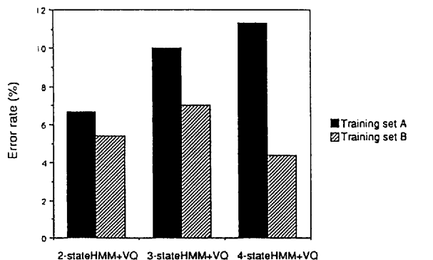
Figure 8. Speaker identification error rate as a function of the number of HMM states.
