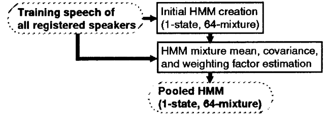
Fig. 2. Block diagram of Method B for making a pooled model.
