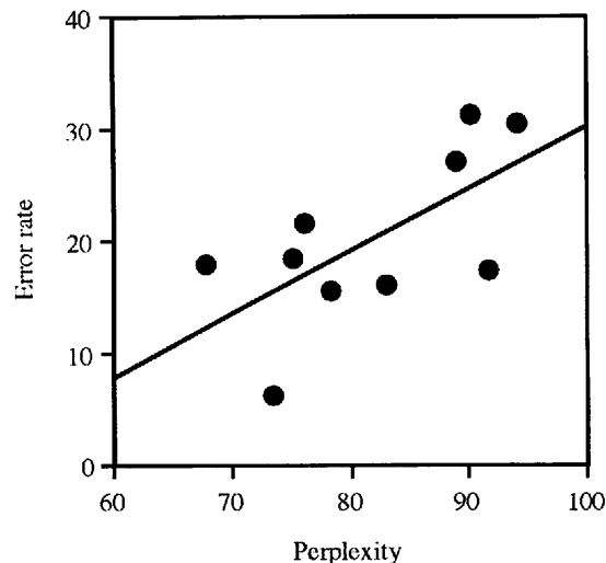
Figure 3 Relation between perplexity and word error rate
