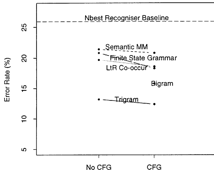
Figure 2. Hypotheses reordering results for the 5 grammar models both with and without the incorporation of the CFG.
