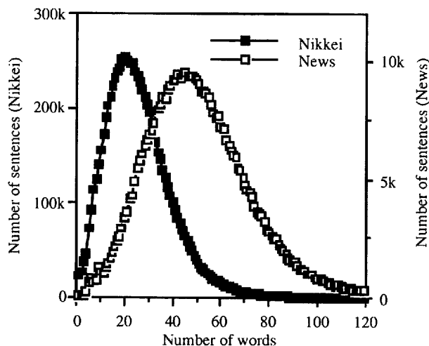
Fig. 2 Histogram of the number of words per sentence
