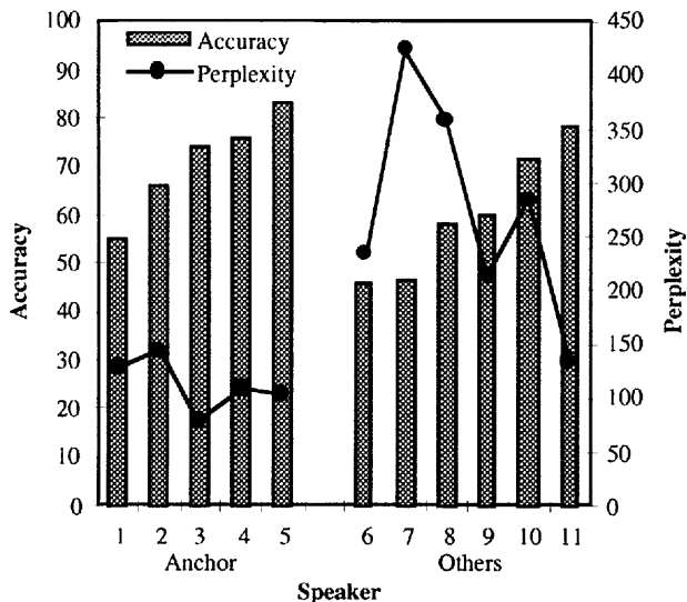
Fig. 3 LVCSR results
