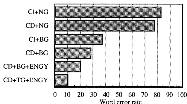
Fig. 1 LV CSR experimental results for newspaper speech. CI: context-independent acoustic models were used, CD: context-dependent acoustic models were used, NG: no grammar models were used, BG: bigram language models were used, TG: trigram language models were used, ENGY: energy parameters were added to the feature parameters.
