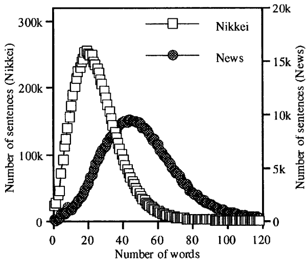
Figure 2: Histogram of the number of words per sentence
