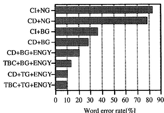
Figure 1: LVCSR experimental results for newspaper speech
