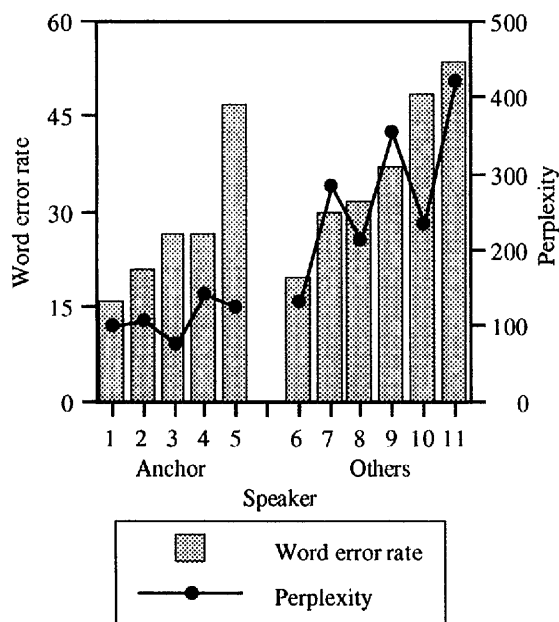
Figure 4: LVCSR results
