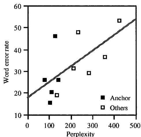
Figure 5: Perplexity vs. Word error rate
