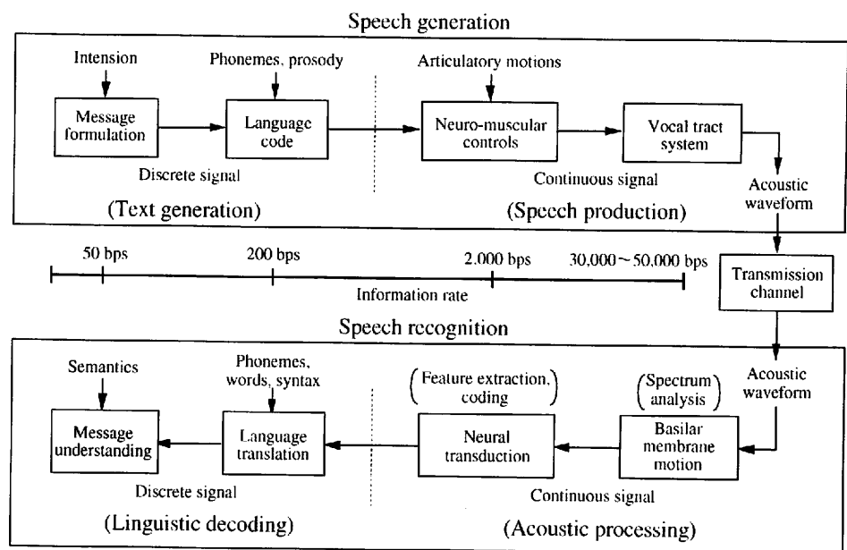
Fig. 3 - Alternative view of speech-production/ speech-perception process
