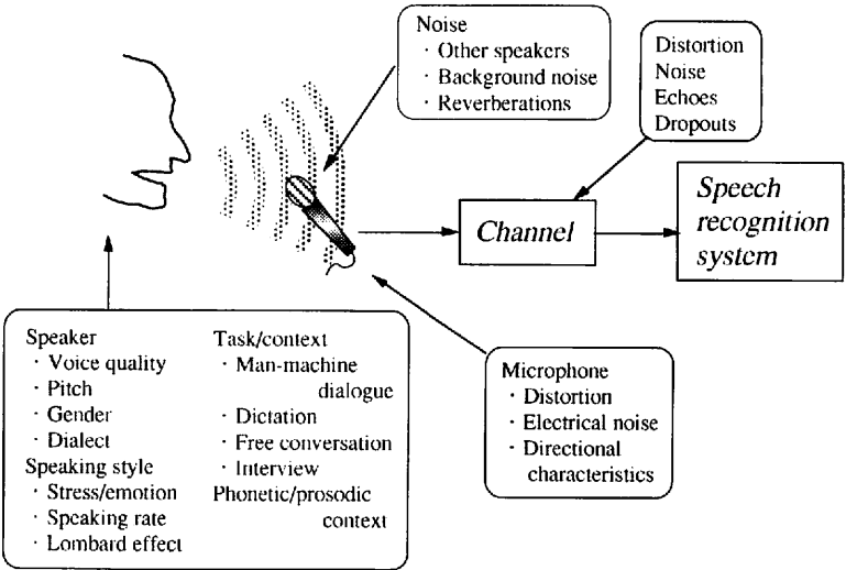
Fig. 5 - Main causes of acoustic variation in speech
