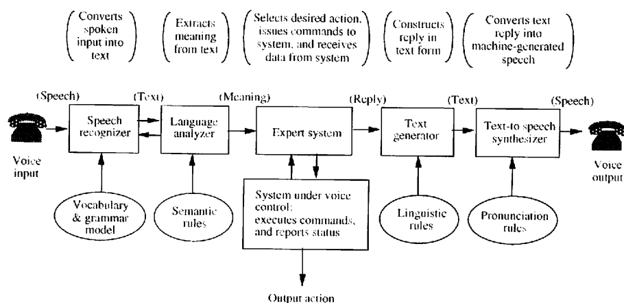
Fig. 1 - Typical structure for task-specific voice control and dialogue systems
