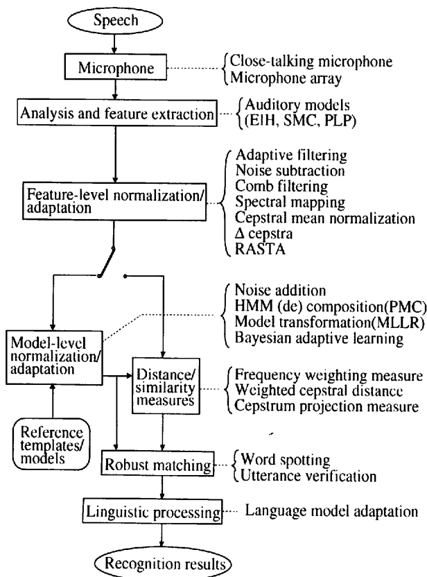
Fig. 6 - Main methods to cope with voice variation in speech recognition
