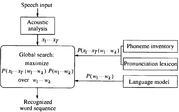
Fig. 4 - Mechanism of state-of-the-art speech recognizers
