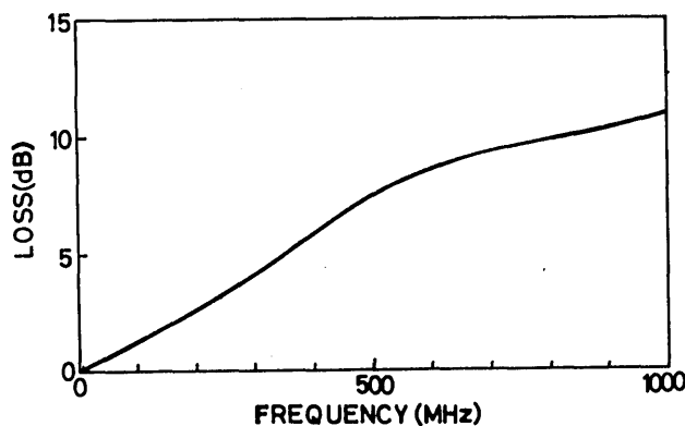
Fig. 8. Baseband frequency response for 100-m long high-N.A. fiber (at 0.82 \mu\text{m} ).
