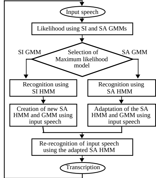
Figure 2. Modified speaker adaptation process (SI: speaker independent, SA: speaker adapted).
