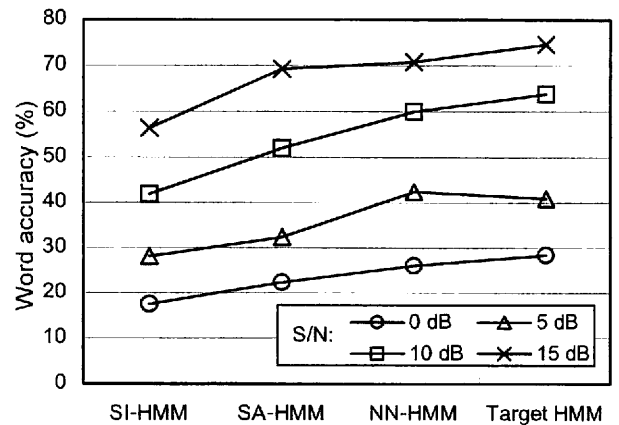
Fig. 3: Word accuracy for same noise conditions as training with different S/N.
