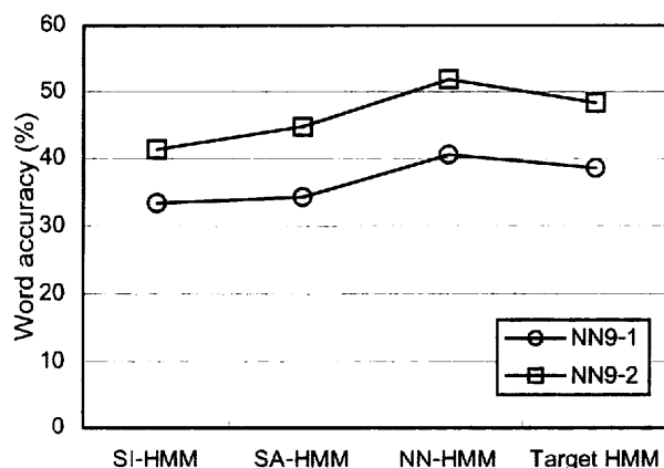
Fig. 5: Word accuracy for test set with same noise and S/N as training.
