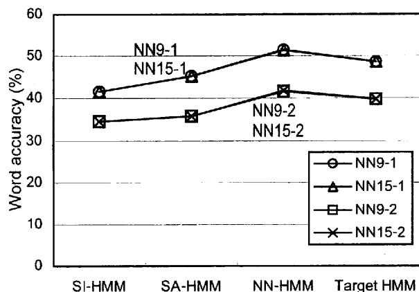
Fig. 7: Word accuracy for test set with noises different from training.
