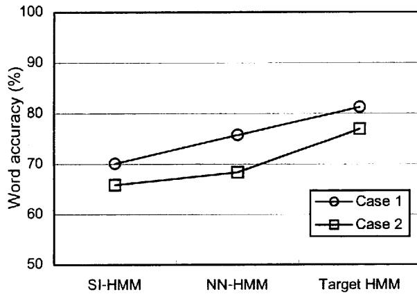
Fig. 11: Word accuracy for test sets.
