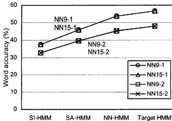
Fig. 4: Word accuracy for noises different from training.
