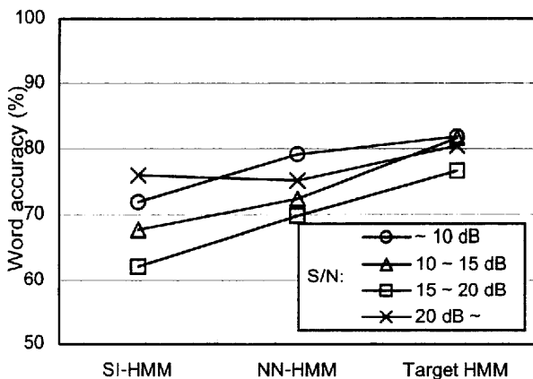
Fig. 12: Word accuracy for test set according to levels of S/N.
