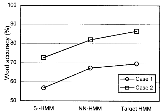
Fig. 10: Word accuracy for training sets.
