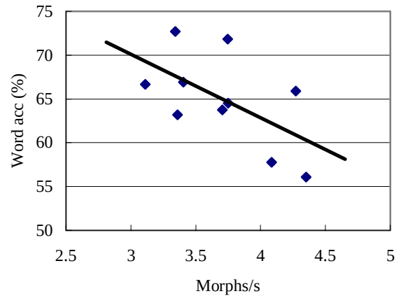
Figure 4. Speaking rate vs. word accuracy.
