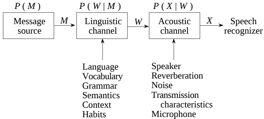
Fig. 6 - A communication-theoretic view of speech generation and recognition.
