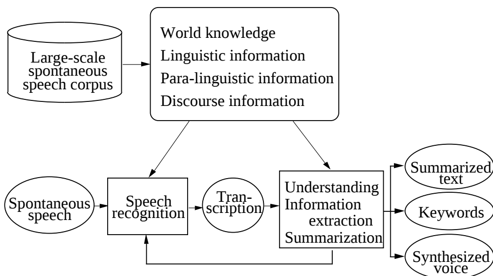
Fig. 7 - Overview of the Japanese national project on spontaneous speech corpus and processing technology.
