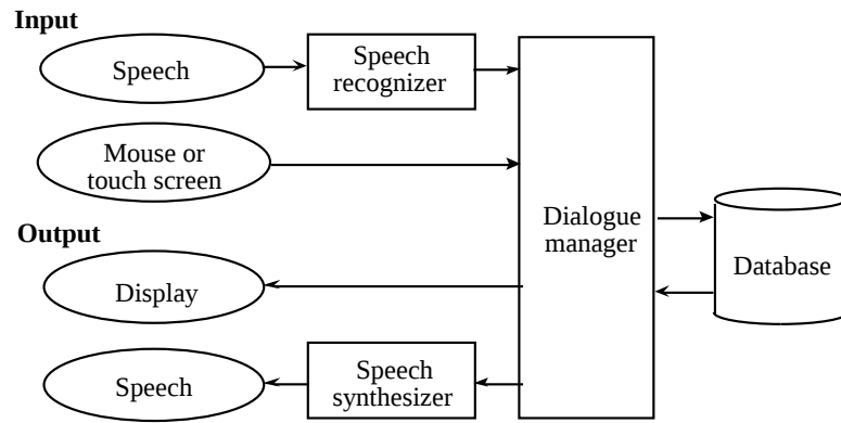
Fig. 3 - Multimodal dialogue system structure for information retrieval.
