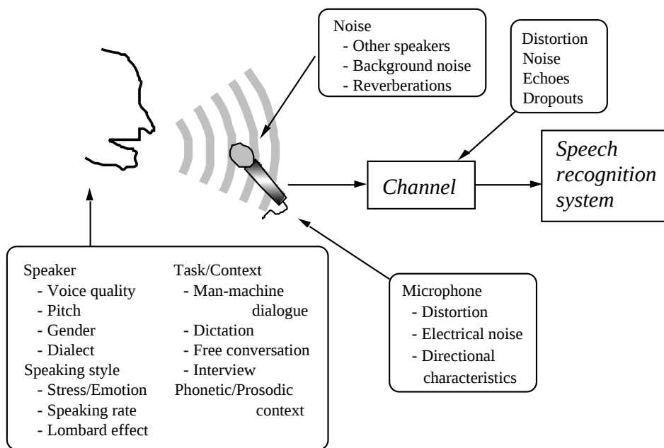
Fig. 2 - Main causes of acoustic variation in speech.
