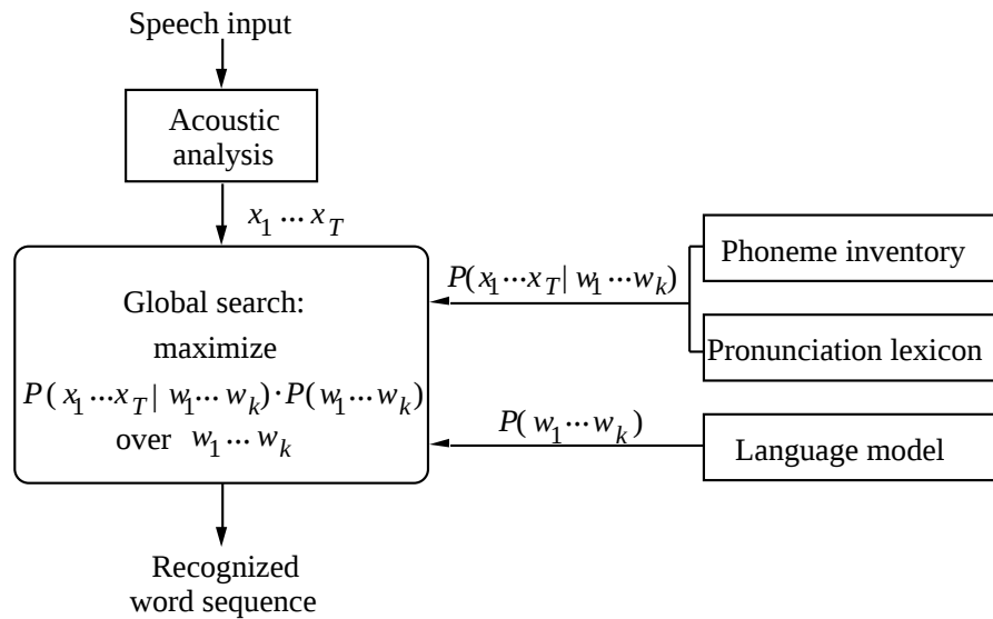
Fig. 1 - Mechanism of state-of-the-art speech recognizers.
