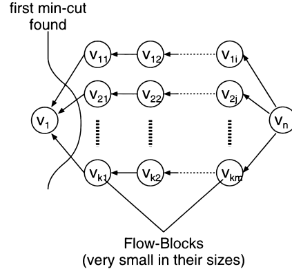
Fig. 6 Example of M(H) where our approach takes a long time to find an optimal cut.
