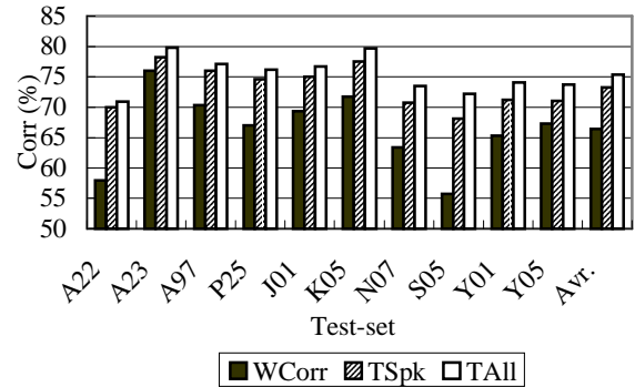
Fig. 3 Recognition and prediction correctness.
