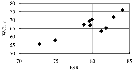
Fig. 5 The predicted success rate ( PSR ) and the recognition correctness.
