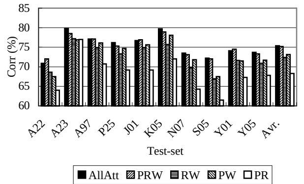
Fig. 4 Analysis of word attributes.
