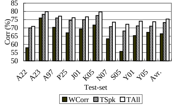
Fig. 3 Recognition and prediction correctness.
