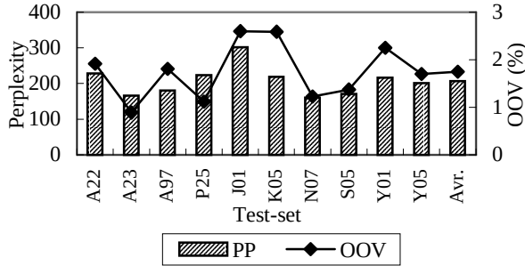
Fig. 1 Test-set perplexity and OOV rate of the task.
