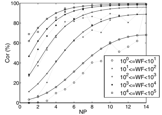
Fig. 2. Word length and recognition correctness.
