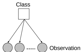
図 4. HMBC (c') equal to classifier (c) but having simpler network structure by using a set of Gaussian mixtures for the Observation node.
