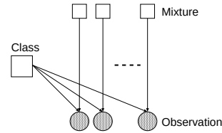
図 1. HMBC (a) using a set of Gaussians for the Observation node.
