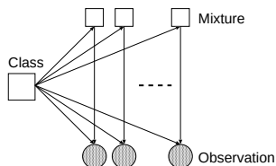
図 3. HMBC (c) using mixture weights depending on classes.
