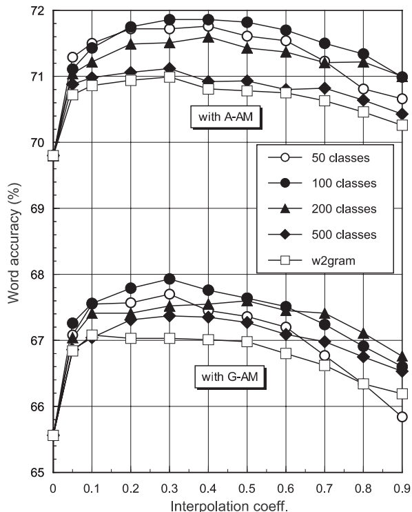
Fig. 4. Word accuracy as a function of the interpolation coefficient \lambda .
