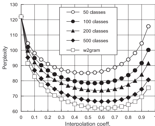
Fig. 3. Test-set word perplexity as a function of the interpolation coefficient \lambda .
