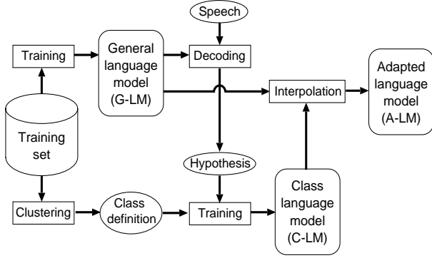
Fig. 1. An overview of the unsupervised class-based language model adaptation method.
