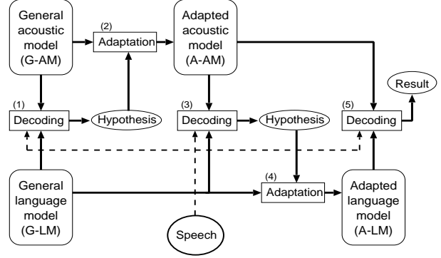
Fig. 2. An overview of the recognition flow using both the proposed language model adaptation and acoustic model adaptation.
