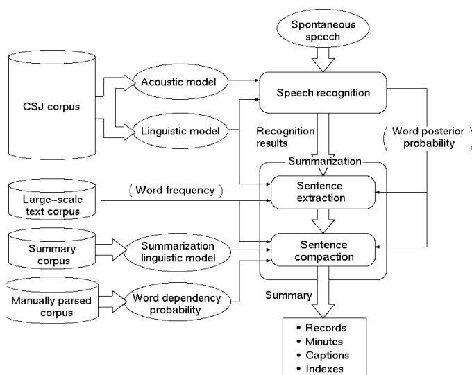
Fig. 5: Automatic speech-to-text summarization system.
