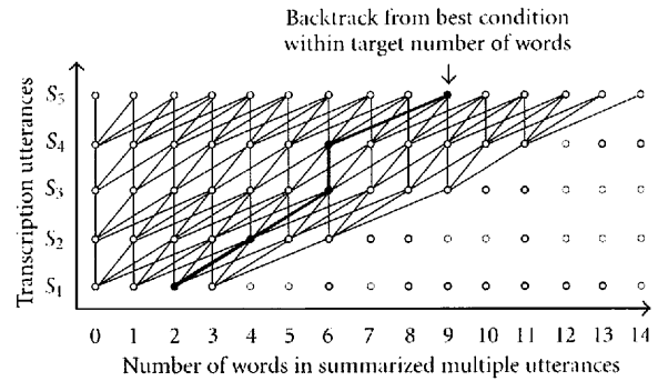
FIGURE 7: Example of two-level DP process to summarize multiple utterances.
