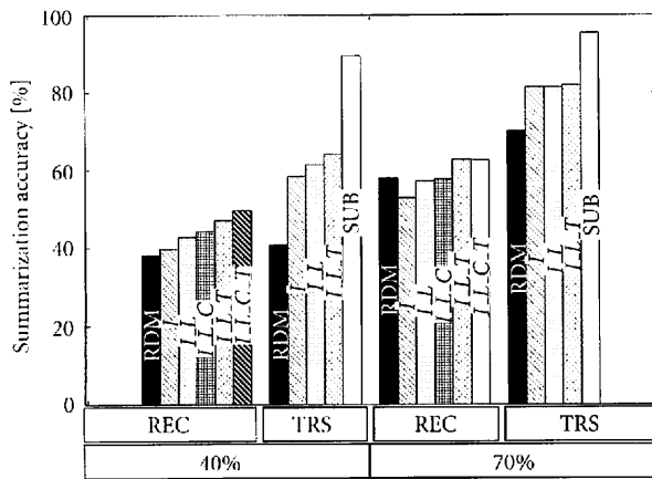
FIGURE 9: Individual utterance summarization at 40% and 70% summarization ratios. REC: summarization of recognition results, TRS: summarization of manual transcriptions, RDM: random word selection, C: confidence score, I : significance score, L : linguistic score, I_L : combination of 2 scores, I_L_C , I_L_T : combination of 3 scores, I_L_C_T : combination of all scores, and SUB: subjective summarization.
