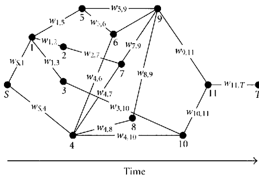
FIGURE 2: Example of word graph.
