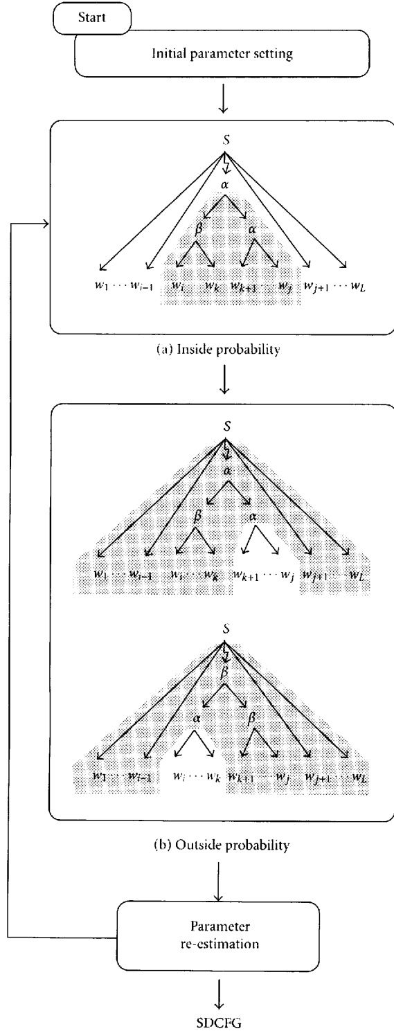
FIGURE 11: Estimation algorithm for SDCFG.
