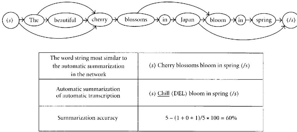
FIGURE 8: Example to calculate summarization accuracy using a word network. The underlined word and <DEL> in automatic summarization represent a substitution error and a deletion error. The summarization accuracy is given by (15).
