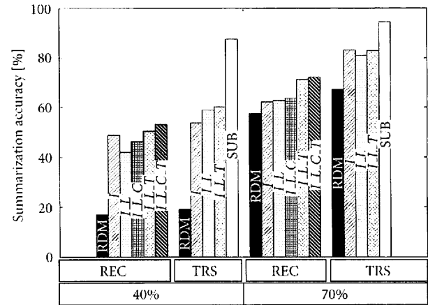
FIGURE 10: Article summarization at 40% and 70% summarization ratios. REC: summarization of recognition results, TRS: summarization of manual transcriptions, RDM: random word selection, C: confidence score, I : significance score, L : linguistic score, I_L : combination of 2 scores, I_L_C , I_L_T : combination of 3 scores, I_L_C_T : combination of all scores, and SUB: subjective summarization.
