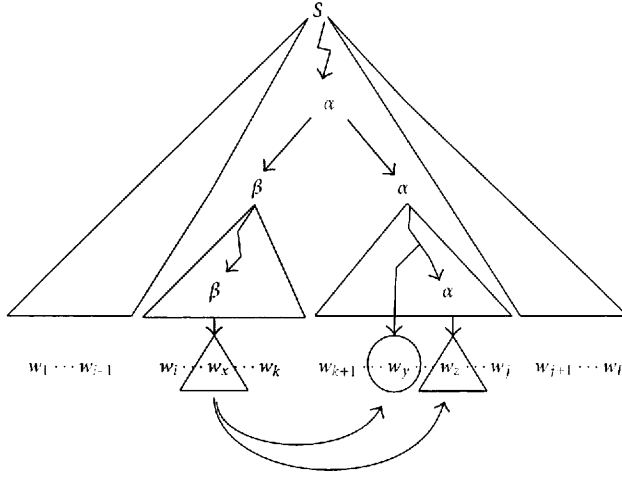
FIGURE 4: Phrase structure tree based on dependency structure.
