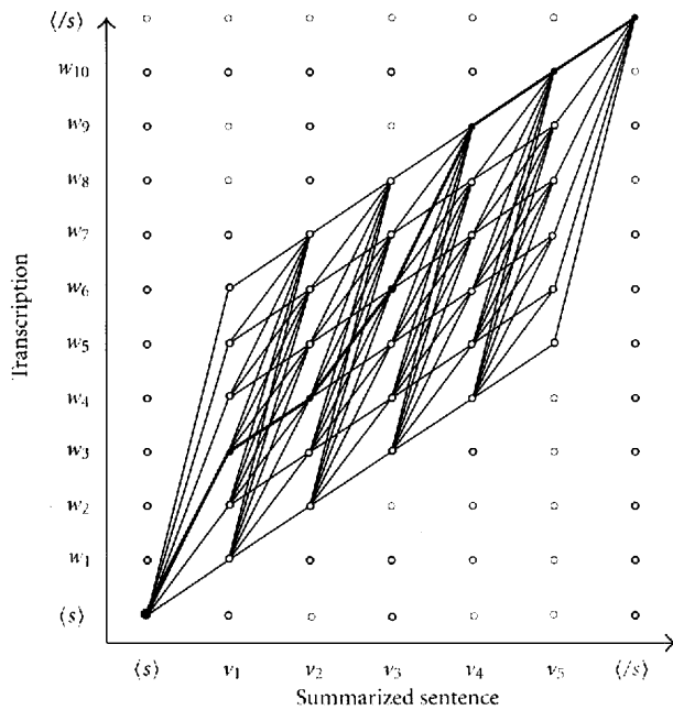
FIGURE 5: Example of DP alignment to summarize an individual utterance.
