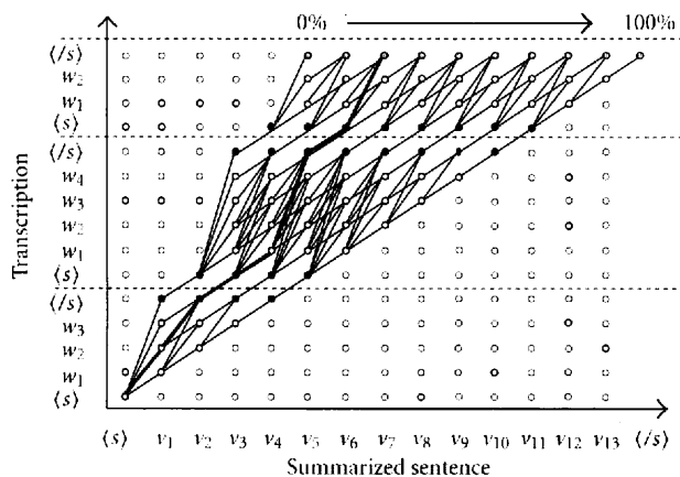
FIGURE 6: Example of DP process to summarize multiple utterances.
