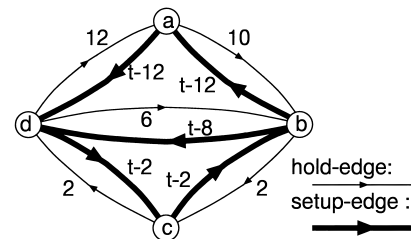
Fig. 2 Constraint graph G_t .
