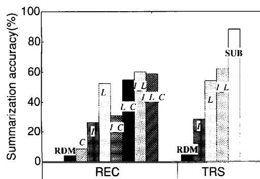
Fig. 4 Summarization at 20% summarization ratio. REC: summarization of recognition, TRS: summarization of manual transcription, RDM: random word selection, C : confidence score, I : significance score, L : linguistic score, I.C , L.C , I.L : combination of 2 scores, I.L.C : combination of all scores, SUB: subjective summarization.
