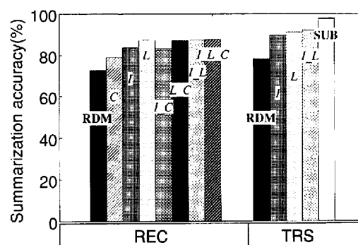
Fig. 8 Summarization at 80% summarization ratio. C : confidence score, I : significance score, L : linguistic score, I.C , L.C , I.L : combination of 2 scores, I.L.C : combination of all scores.
