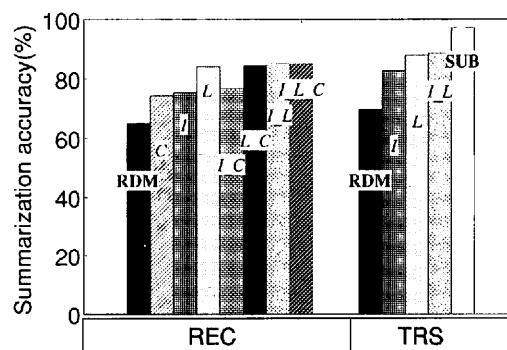
Fig. 7 Summarization at 70% summarization ratio. C : confidence score, I : significance score, L : linguistic score, I.C , L.C , I.L : combination of 2 scores, I.L.C : combination of all scores.
