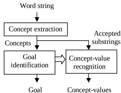
Figure 1. Overall architecture of the multi-stage SLU.
