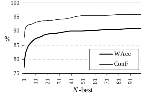
Figure 6. WAcc and ConF results with respect to values of N in an oracle test for the DS set.
