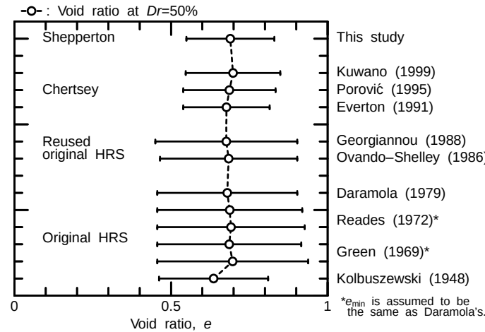
Fig. 7: Maximum and minimum void ratios
