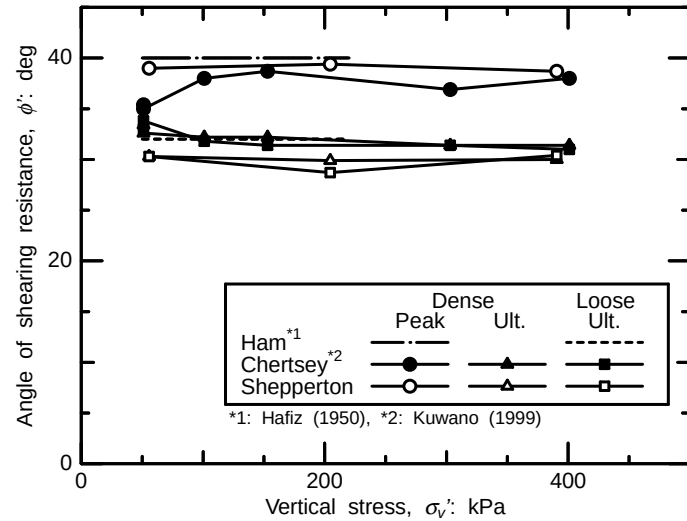
Fig. 8: Angles of shearing resistance in direct shear box test
