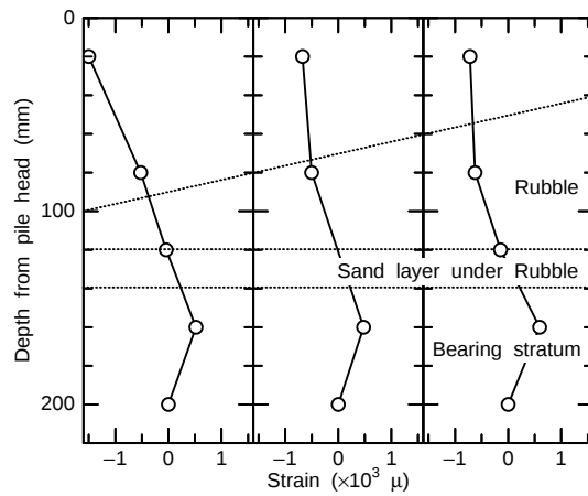
Fig. 17. Permanent strain distributions of pile in PW2.
