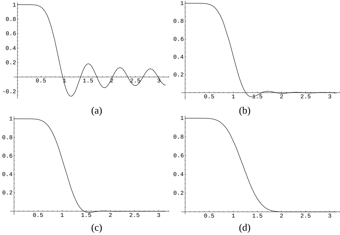
Fig. 2. Plots of P_{3,m,10}(\sin^2 \frac{\omega}{2}) . (a) m=0 . (b) m=5 . (c) m=10 . (d) m=50 . The horizontal axis depicts the normalized frequency \omega .
