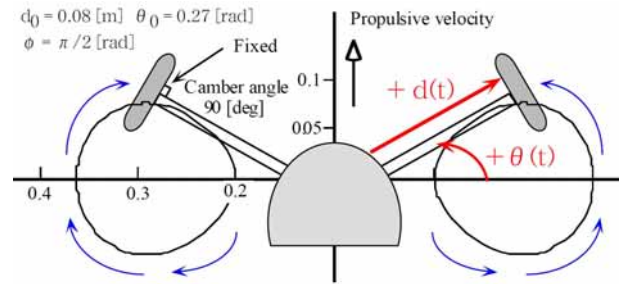
Fig.2 Simulation model
