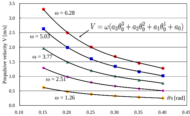
Fig.3 Simulated propulsive velocity with paramter \theta_0 and \omega
