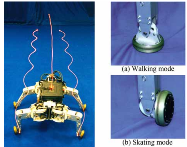
Fig.1 Roller-Walker
