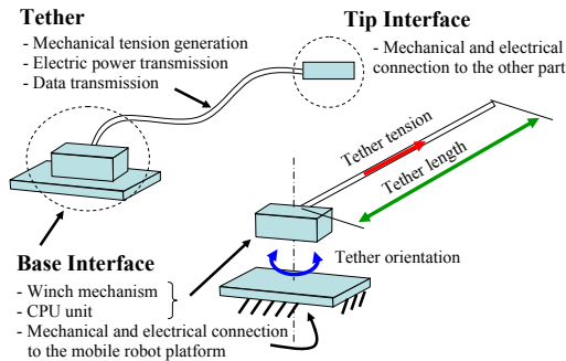
Fig. 2 Hyper-Tether Concept
