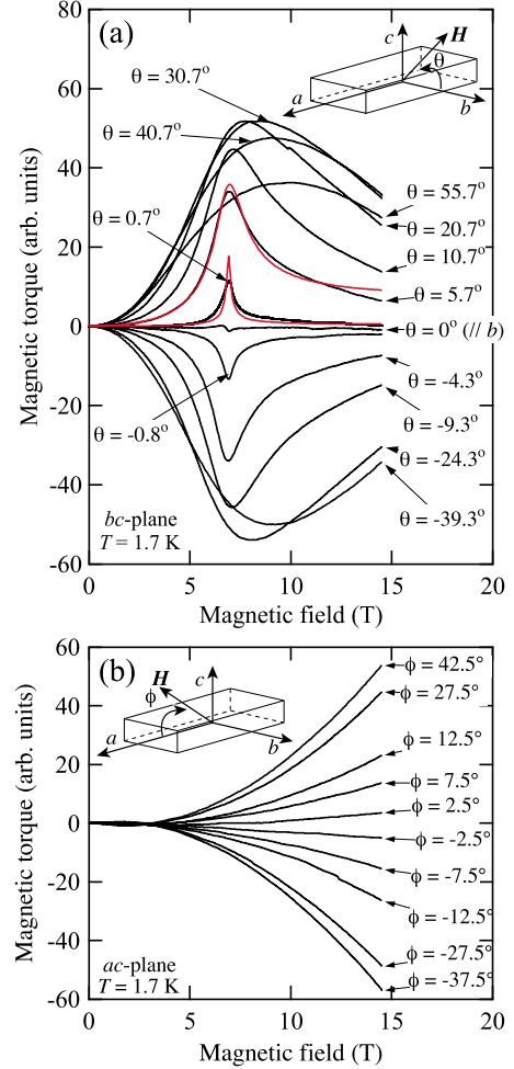
FIG. 2. (Color online) Magnetic torque curves of (MDT-TS)(AuI 2 ) 0.441 at 1.7 K under various magnetic field directions of \theta and \phi , which are the angles tilted (a) from b to c and (b) from a to c axes, respectively. The red lines in (a) are the fitted results.
