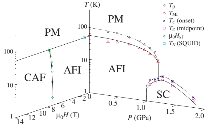
FIG. 5. (Color online) Phase diagram of (MDT-TS)(AuI 2 ) 0.441 (PM: paramagnetic metal, AFI: antiferromagnetic insulator, SC: superconductor, CAF: canted antiferromagnetic state). The solid and dotted lines are guides to the eye.
