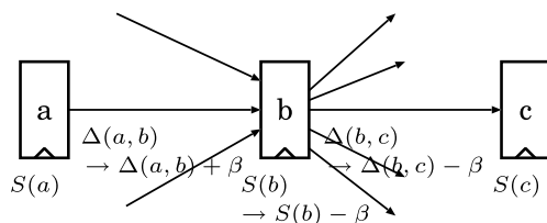
Fig. 7 The changed slack after clock schedule modification.
