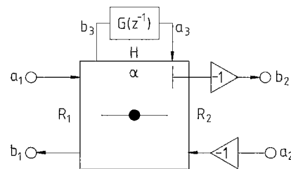
Fig. 2 Digital series section.
