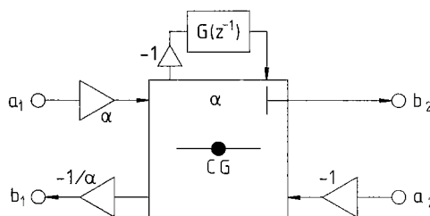
Fig. 12 Parallel section with a series CG-adaptor.
