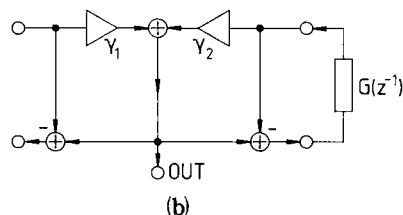
Fig. 9 (a) New port matching scheme. (b) Its internal circuit.
