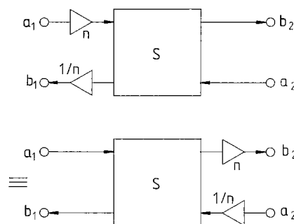
Fig. 13 Transformation of multiplier movement.
