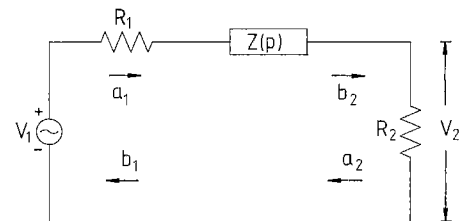
Fig. 1 Analog series section.
