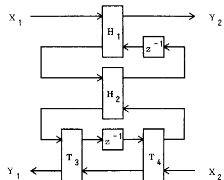
Fig. 10 Realization of the second-degree section.
