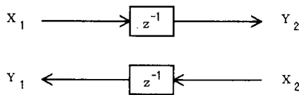
Fig. 2 Lossless digital two-port defined by Eq. (11).
