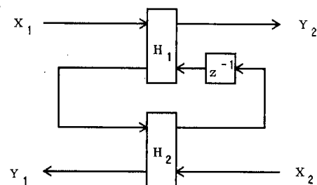
Fig. 8 Realization of the first-degree section.
