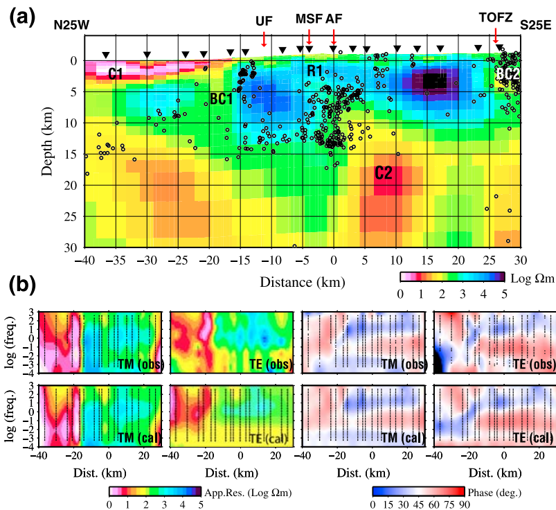
Figure 3. (a) Two-dimensional resistivity model obtained along the 70 km MT profile across the NKTZ. Inverted triangles indicate the locations of the MT sites. Seismic activity located close to the study area [Ito et al. , 2007], within \pm 10 km of the section line, is shown by open circles. Red arrows with abbreviations indicate the locations of the surface traces of active faults. Features labeled C1, C2, R1, BC1, and BC2 are discussed in the text. (b) MT pseudo-sections of the (top) observed responses and (bottom) calculated responses from the final model. Dots represent the data used in the inversion procedure.
