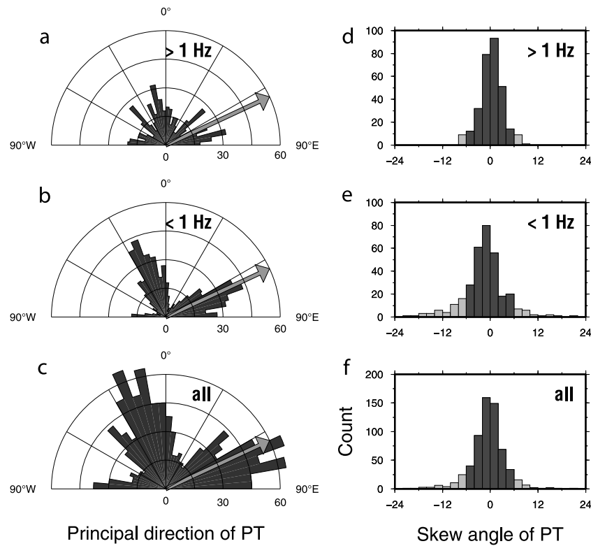
Figure 2. Rose diagrams and histograms of directional parameters for the respective frequency bands. (a–c) Cumulative principal directions ( \alpha ) of the phase-tensor (PT) analysis [Caldwell et al. , 2004] are shown with a 90^\circ ambiguity. The estimated strike for modeling, N65^\circ E , is indicated by arrows. (d–f) Cumulative skew angles ( \beta ) of the PT, which represent the asymmetry of the phase response produced by the three-dimensional structure. The data have sizable \beta values ( |\beta| > 6^\circ ), shown as gray bars, which placed a limit on the use of the inversion procedure.
