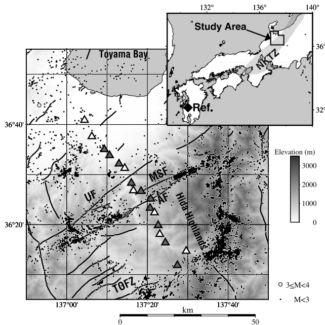
Figure 1. Topographic map of the study area. The epicenters of microearthquakes determined by the Kamitakara Observatory (DPRI, Kyoto University Japan) are plotted as circles scaled to earthquake magnitude (for the period January 2000 to May 2004). Several active faults are shown as thick lines. Gray and white triangles represent five/four-component magnetotelluric (MT) sites and electric-field-only MT sites, respectively. The NKTZ [Sagiya et al. , 2000] is shown as the shaded area in the inset map. The black diamond indicates the remote reference site employed for MT data processing.
