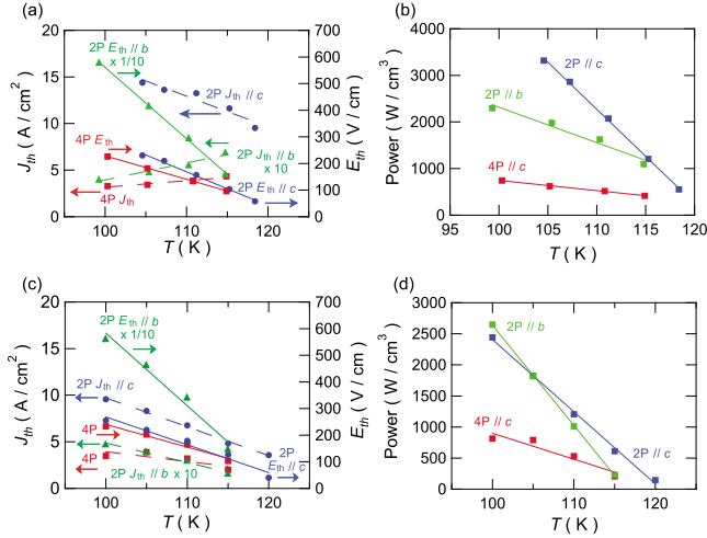
FIG. 4. (Color online) Temperature dependence of observed and simulated threshold currents, fields, and power in \beta'' -(BEDT-TTF) 3 (HSO 4 ) 2 . (a) Observed temperature dependence of J_{th} and E_{th} extracted from Figs. 2(a)–2(c). Solid lines are for E_{th} and dashed lines for J_{th} . (b) Observed temperature dependence of the applied power J_{th} \times E_{th} at the threshold, estimated from (a). (c) Simulated J_{th} and E_{th} extracted from Figs. 2(a)–2(c). Solid lines for E_{th} and dashed lines for J_{th} . (d) Simulated threshold power J_{th} \times E_{th} estimated from (c).
