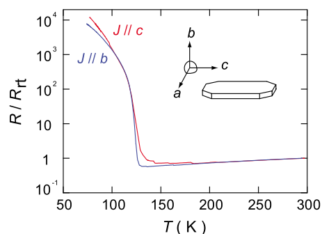
FIG. 1. (Color online) Temperature dependence of in-plane ( \parallel c ) and out-of-plane ( \parallel b ) resistivities of \beta'' -(BEDT-TTF) _3 (HSO _4 ) _2 . The room-temperature resistivities are 0.028 \Omega cm along c and 8.26 \Omega cm along b .
