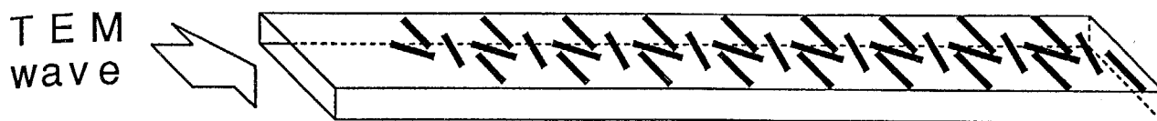
Fig. 7-10. 1-dimensional array.
