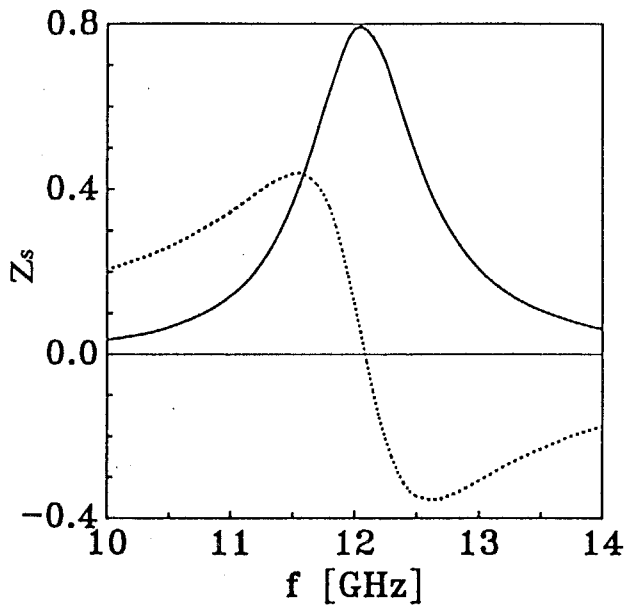
Fig. 3-4. Frequency characteristics of Z_s .
