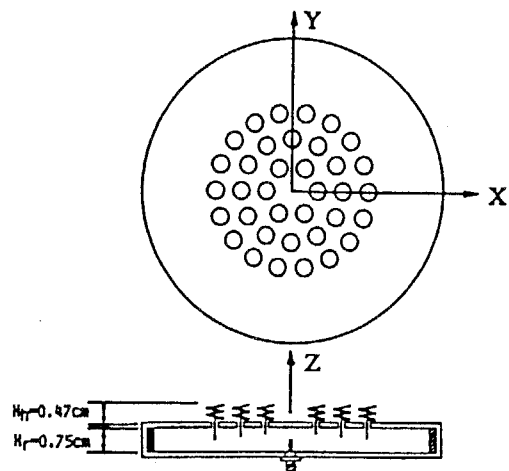
(h) Helical array fed by radial line (RLH) (from Nakano, et. al. [16]).
