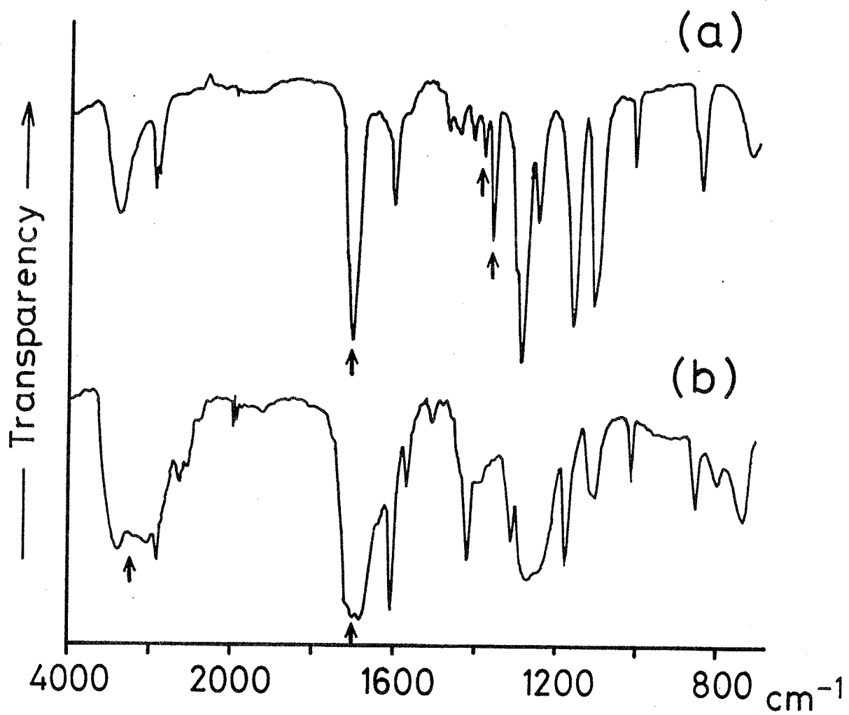
Figure 3-6. IR spectra of poly(1e) (a) and poly(2) (b). The full elaboration on the absorption bands indicated by arrows is described in the Results and Discussion.
