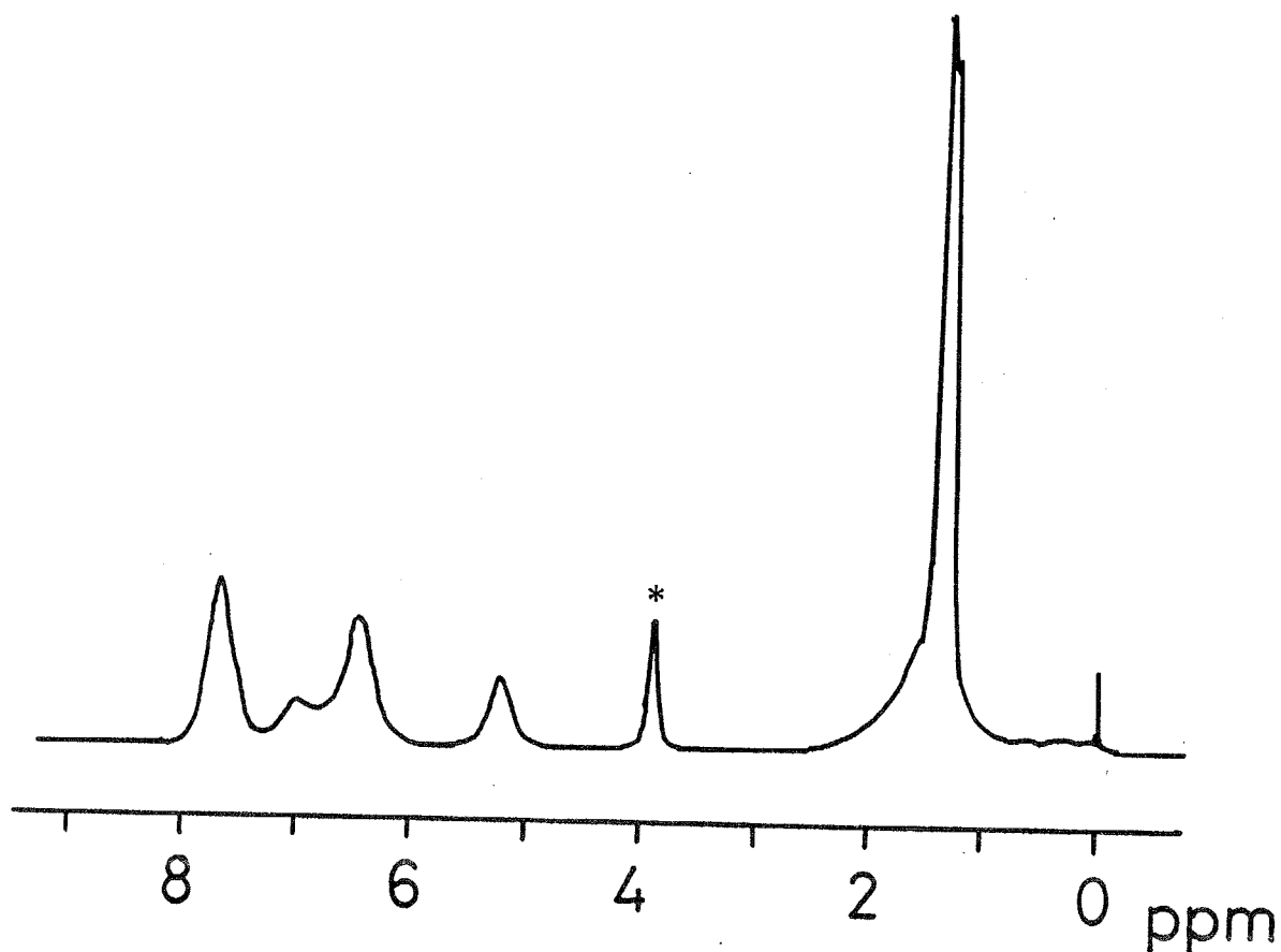
Figure 3-1. 1 H NMR spectrum of poly( 1d ). Peak attributable to methyl ester is marked with an asterisk (*).
