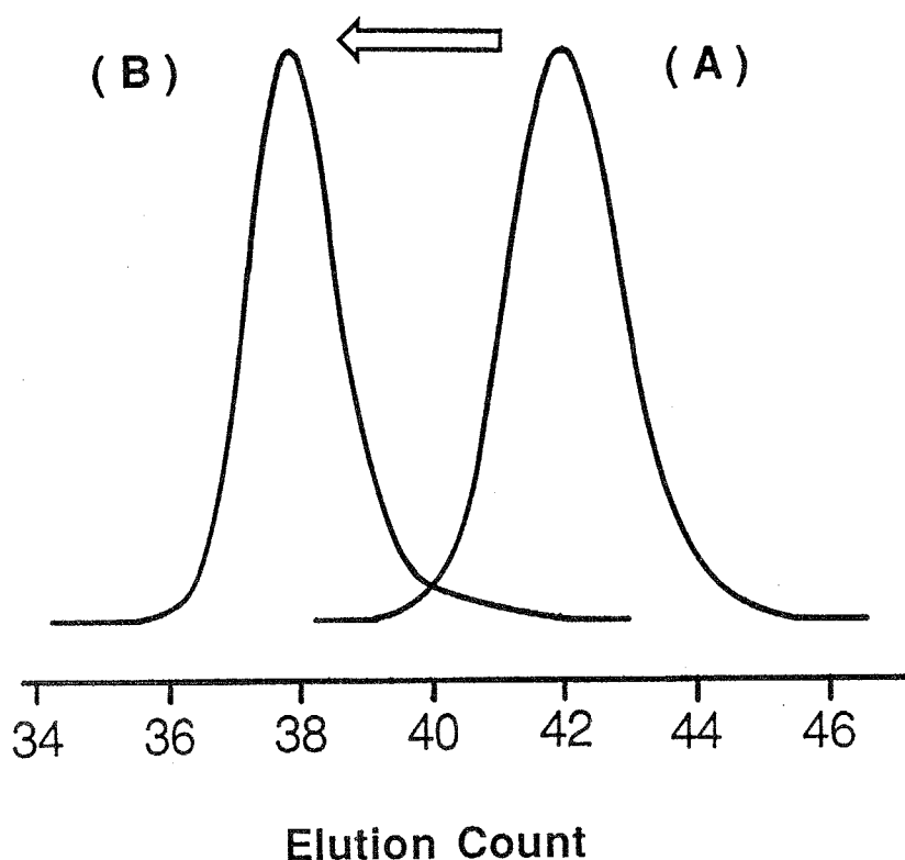
Figure 4-1. SEC curves of poly(1)s obtained at -78^{\circ}\text{C} : (A) the first-stage polymerization, M_n(\text{obsd}) = 7500 , M_w/M_n = 1.05 ; (B) the second-stage polymerization, M_n(\text{obsd}) = 18\,000 , M_w/M_n = 1.04 (the second feed of monomer was added 30 min after the first-stage polymerization).
