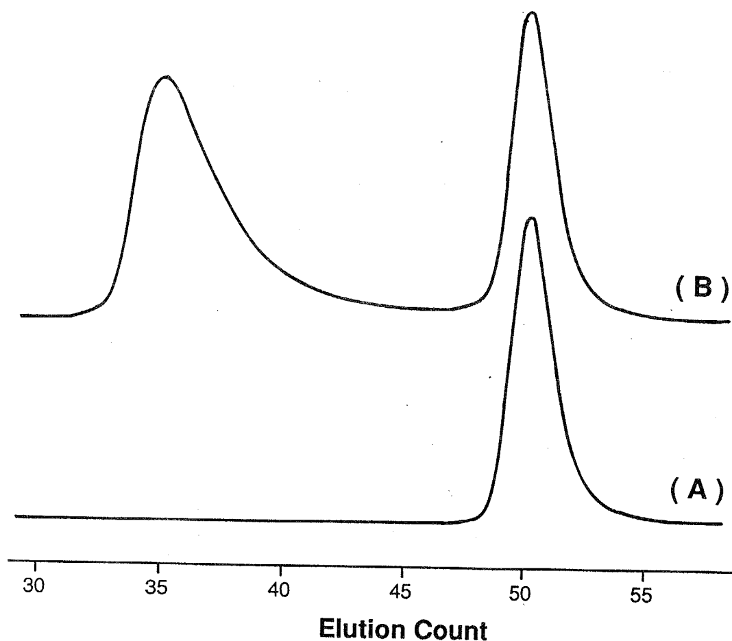
Figure 7-4. SEC curves (THF) of poly(1) at the first-stage polymerization (A) and of the copolymerization product after the second-stage polymerization of styrene in THF at -78^{\circ}C for 2 h (B) (Table 7-4, run 42): peak A, M_n(\text{obsd}) = 12\ 000 , M_w/M_n = 1.09 .
