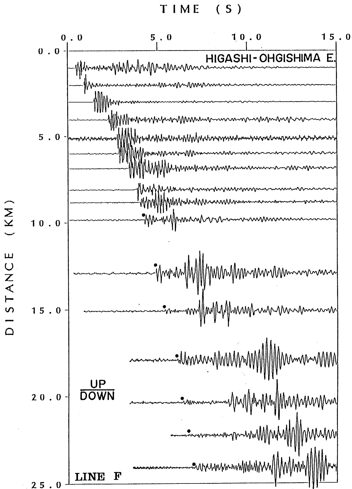
Fig. 2-23a. Observed seismograms at the stations along the Higashiohgishima-Okazu line (Line F in Fig. 2-1) during the Higashiohgishima explosion. Each trace indicates vertical ground velocity and is normalized to its maximum amplitude. Each solid circle shows onset of initial phase.
