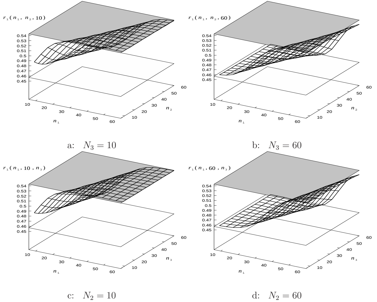
Figure 6.2: r_1(n_1, N_2, n_3) behavior in E_2/H_2/1 \rightarrow /E_2/1 \rightarrow /H_2/1 ( \rho_1 = 0.6, \rho_2 = 0.8, \rho_3 = 0.4 )
