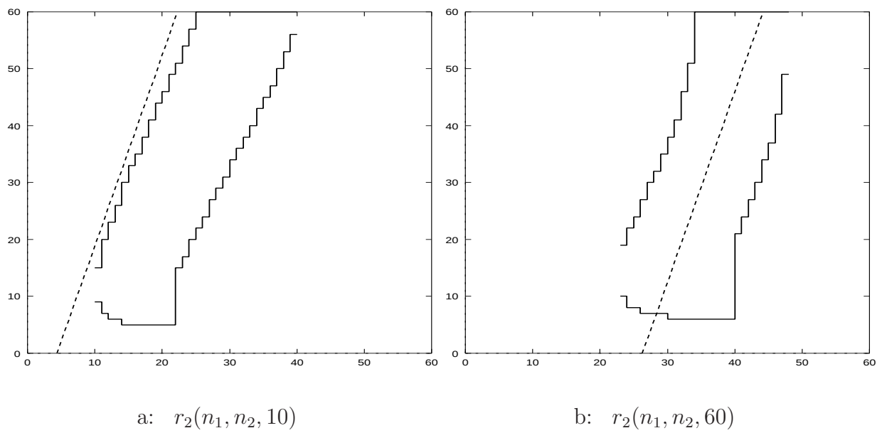
Figure 6.5: Characterization of r_2(n_1, n_2, N_3) surface
