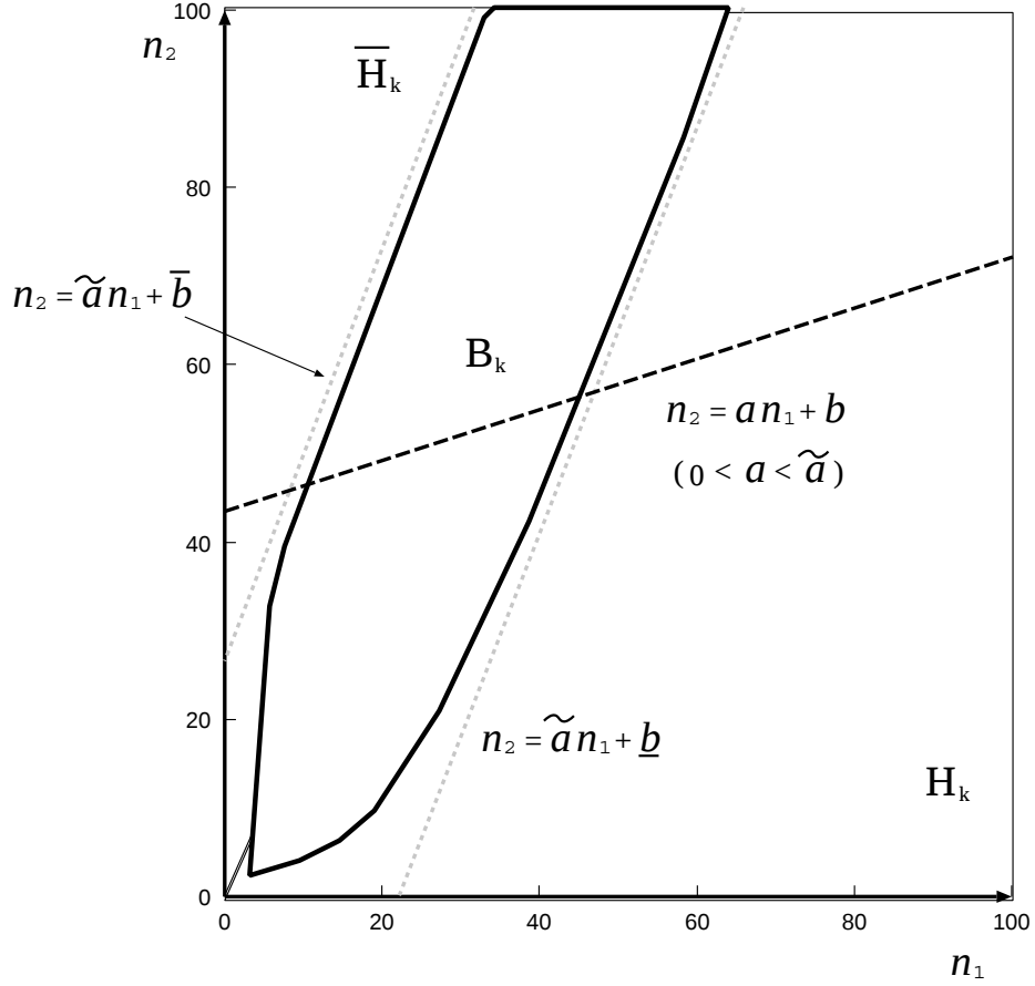
Figure 2.4: constraint lines for band B_k
