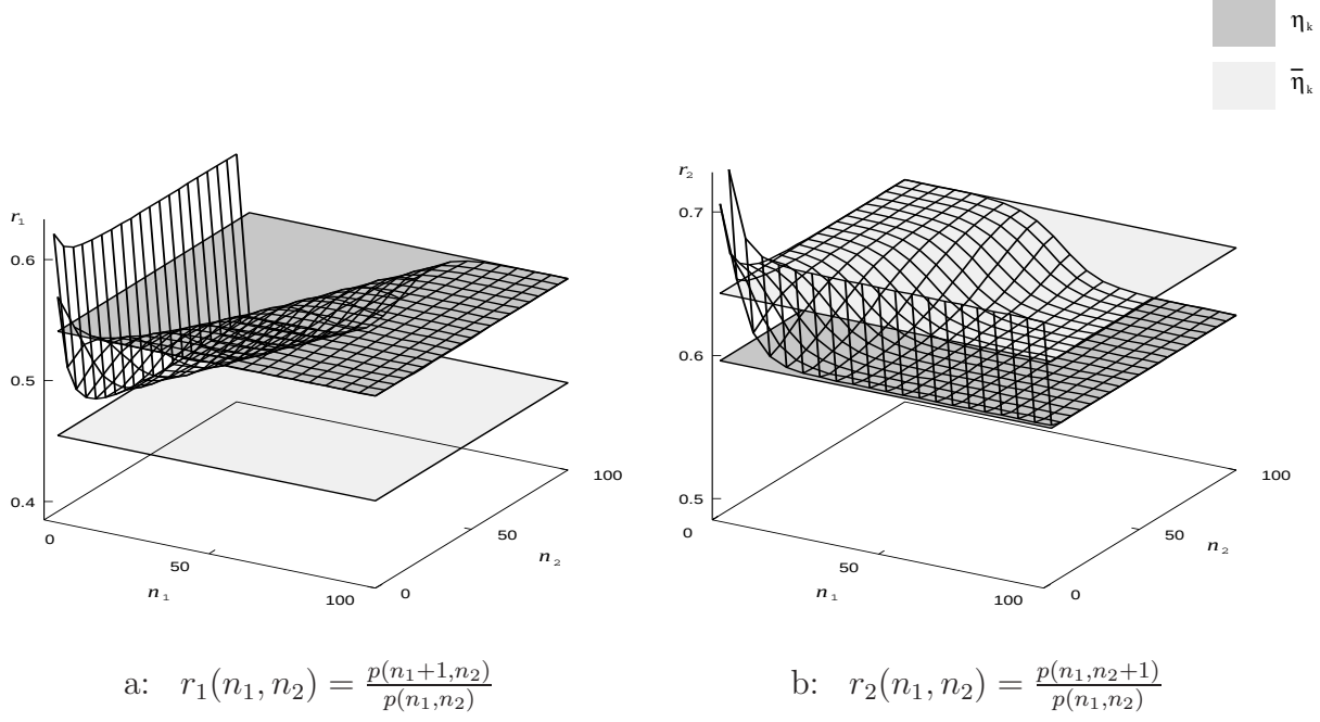
Figure 2.2: r_k behavior in E_2/H_2/1 \rightarrow /E_2/1 ( \rho_1 = 0.6, \rho_2 = 0.8 )
