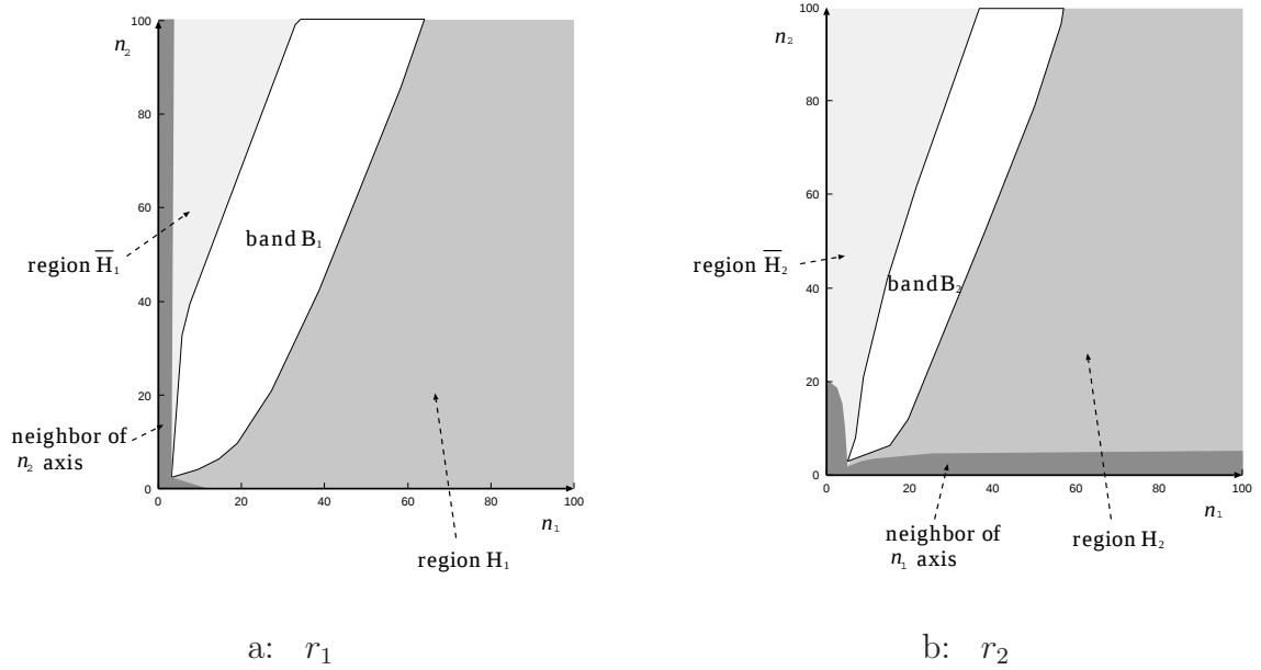
Figure 2.3: Characterization of r_k surface
