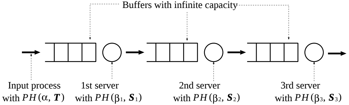
Figure 6.1: Three-stage tandem queueing system
