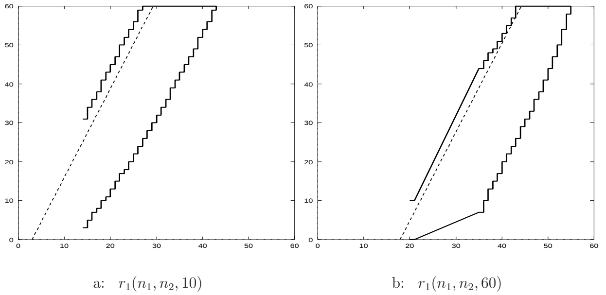
Figure 6.3: Characterization of r_1(n_1, n_2, N_3) surface
