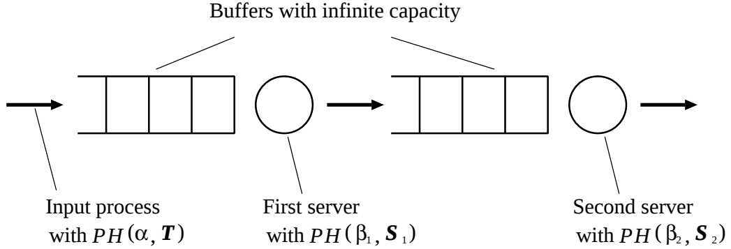
Figure 4.1: Two-stage tandem queueing system
