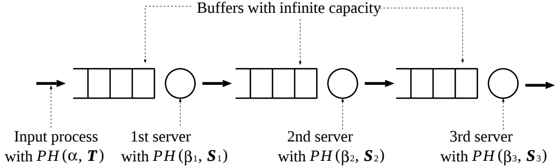
Figure 5.1: Three-stage tandem queueing system
