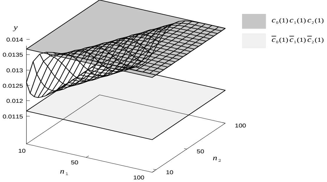
Figure 2.6: Behavior of y(1, 1, 1|n_1, n_2) in E_2/H_2/1 \rightarrow /E_2/1 with \rho_1 = 0.6, \rho_2 = 0.8
