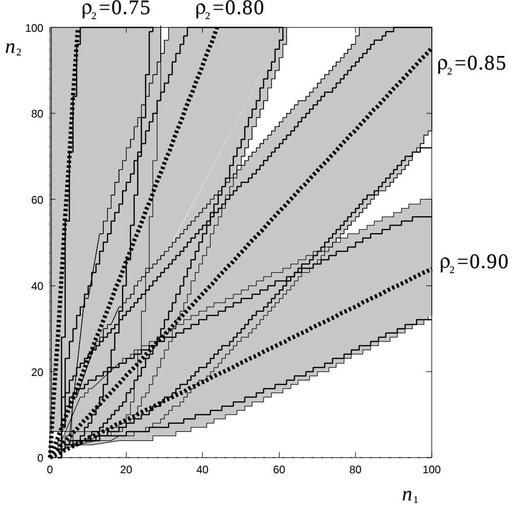
Figure 2.9: Movement of B_1 and B_2 in E_2/H_2/1 \rightarrow /E_2/1 with \rho_1 = 0.6
