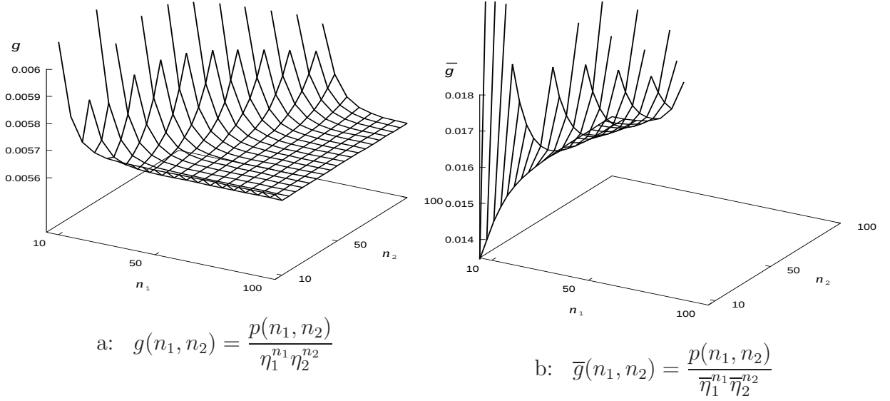
Figure 2.5: Behaviors of g(n_1, n_2) and \bar{g}(n_1, n_2) in E_2/H_2/1 \rightarrow /E_2/1 with \rho_1 = 0.6, \rho_2 = 0.8
