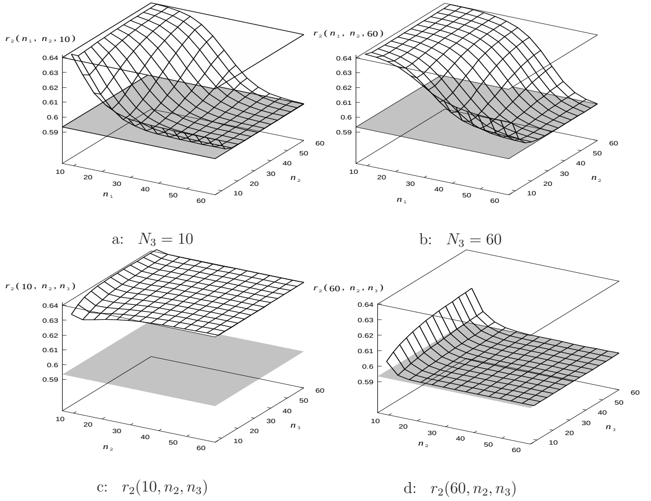
Figure 6.4: r_2 behavior in E_2/H_2/1 \rightarrow /E_2/1 \rightarrow /H_2/1 ( \rho_1 = 0.6, \rho_2 = 0.8, \rho_3 = 0.4 )
