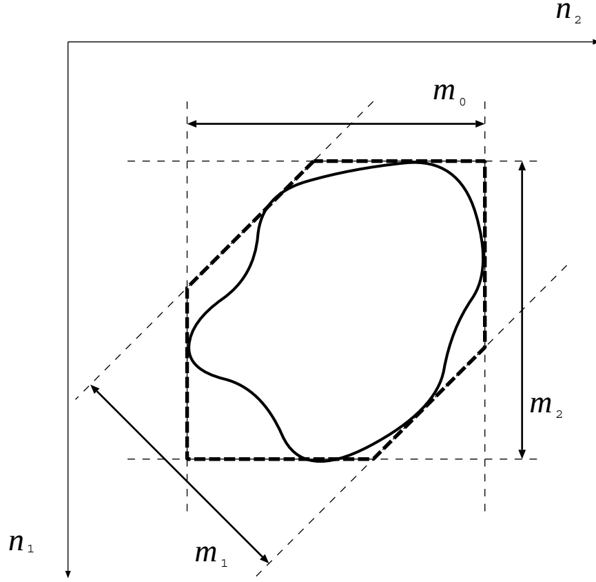
Figure 5.6: Diameters of a set
