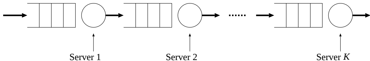
Figure 1.1: A tandem queueing system
