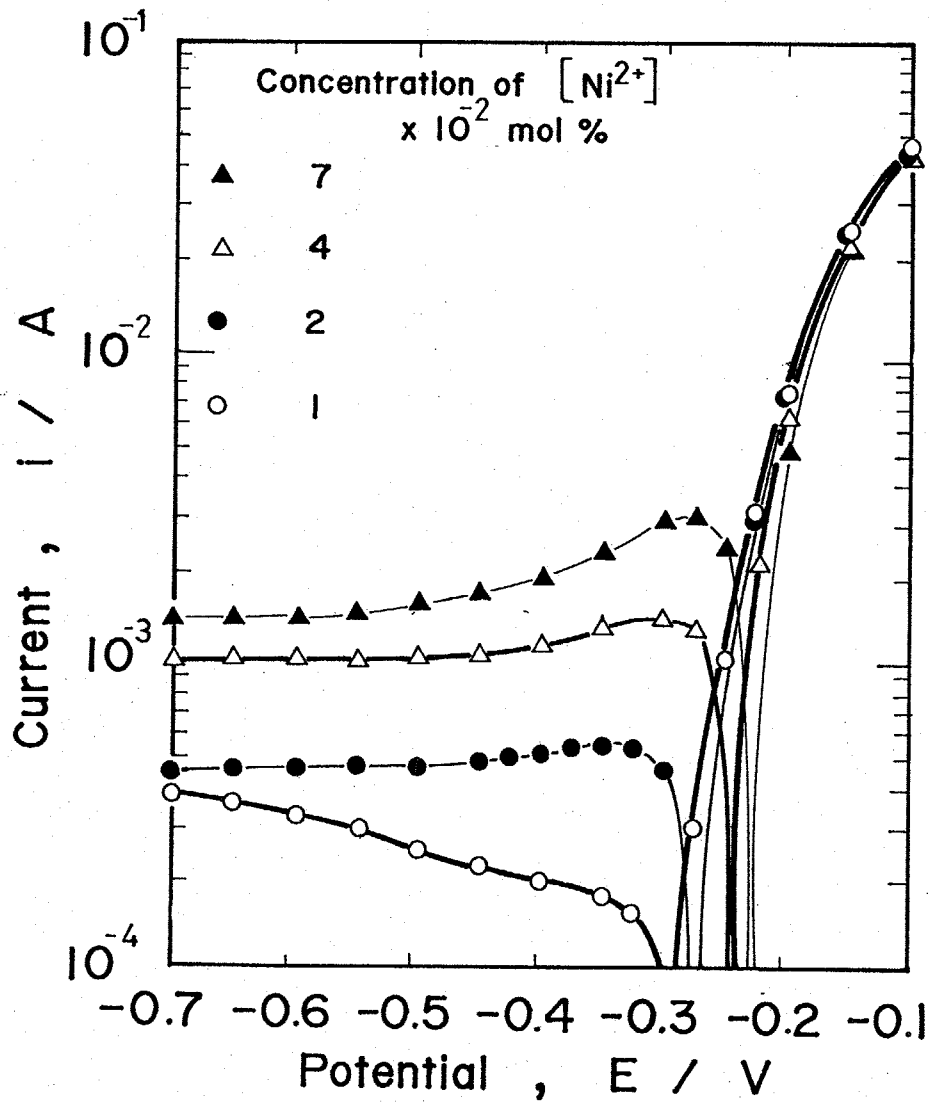
Fig. 2-6 Polarization curves of Ni in LiCl-KCl melts at 773K. Electrode surface area ; 2.4 \times 10^{-5} m^2 . Sweep rate ; 0.020V/s.
