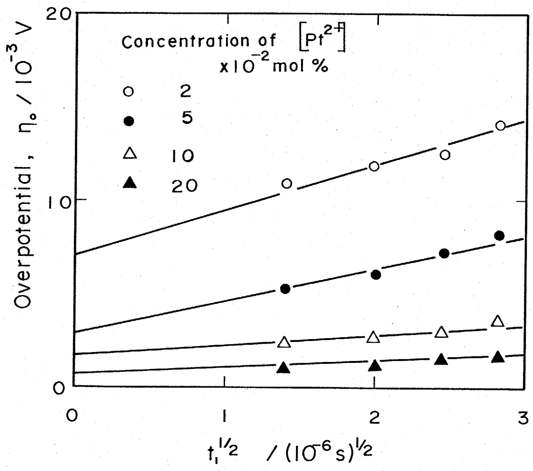
Fig. 2-23 Plots of overpotential \eta_0 against t_1 for Pt/Pt 2+ electrode in LiCl-KCl melts at 773K, i_2 = 3 \times 10^3 A/m^2 .
