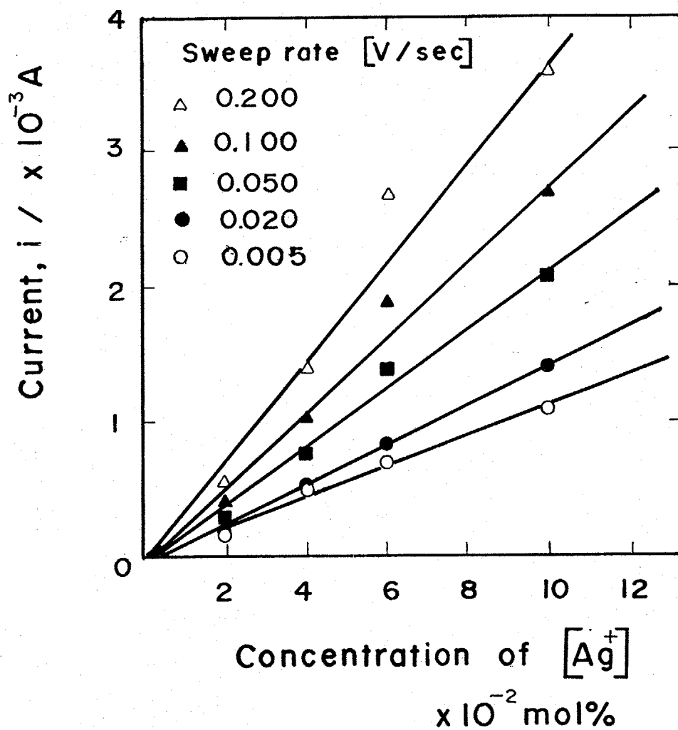
Fig. 2-13 Dependence of cathodic peak current on concentration of [\text{Ag}^+] in LiCl-KCl melts at 773K.
