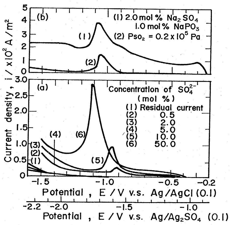
Fig. 4-1 Cathodic polarization curves of Ni in NaCl-KCl melt at 973K. Sweep rate ; 0.010 V/s
