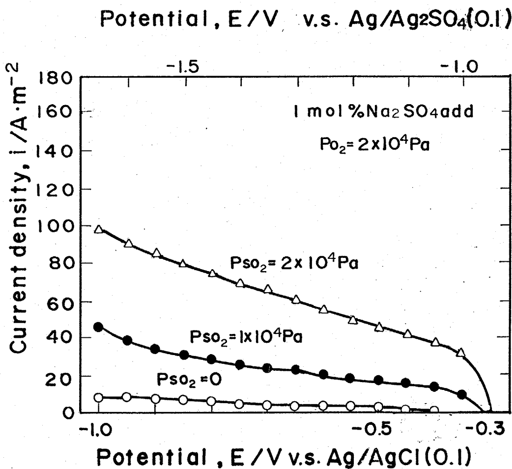
Fig. 4-8 Effect of P_{SO_2} on cathodic polarization curves of Ni in NaCl-KCl containing Na 2 SO 4 (1mol%) at 973K. Sweep rate ; 0.010V/s.
