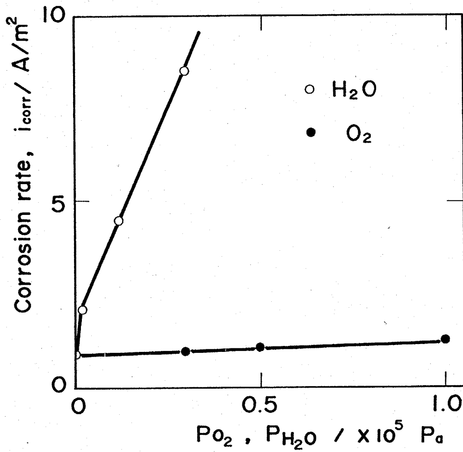
Fig. 4-15 Effect of P_{\text{O}_2} and P_{\text{H}_2\text{O}} on corrosion rate of Ni in \text{Na}_2\text{SO}_4 - \text{Li}_2\text{SO}_4 melt at 973K.
