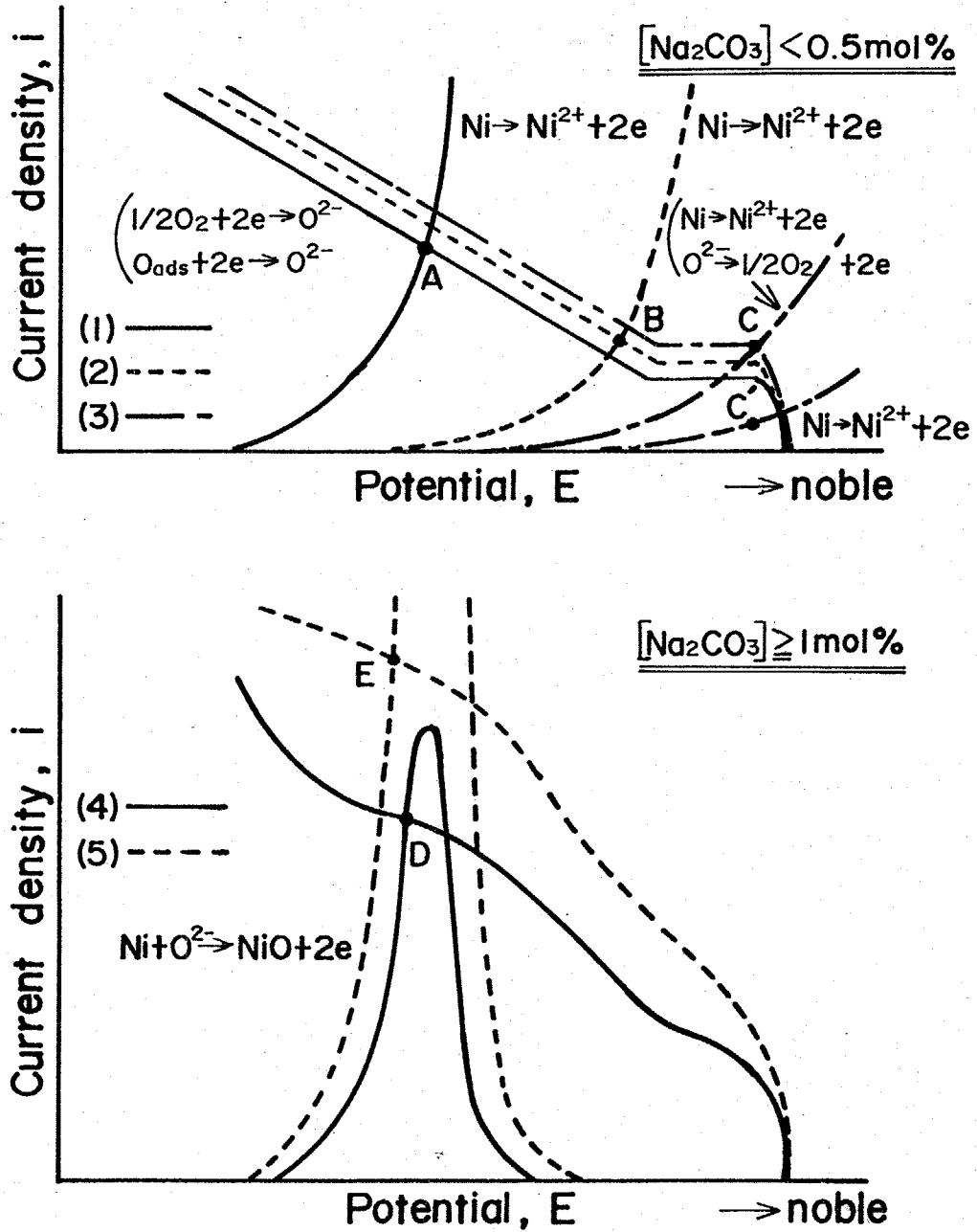
Fig. 3-8 Schematic diagrams of partial polarization curves for Ni in NaCl-KCl containing carbonate ion. P_{O_2} = 1 \times 10^5 \text{ Pa} , Concentration of carbonate ion; (1) < (2) < (3) < (4) < (5).
