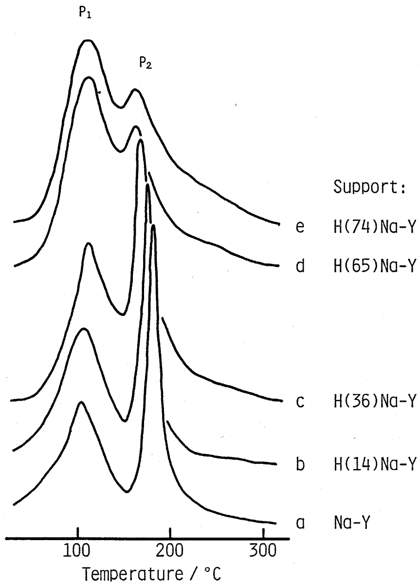
Fig. 3 CO desorption profiles during temperature programmed decomposition of \text{Mo}(\text{CO})_6/\text{Y} zeolites
