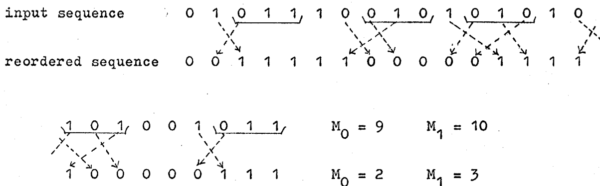
Fig. 2. An example of Policy I_0 with the restriction R_1 for k=3
