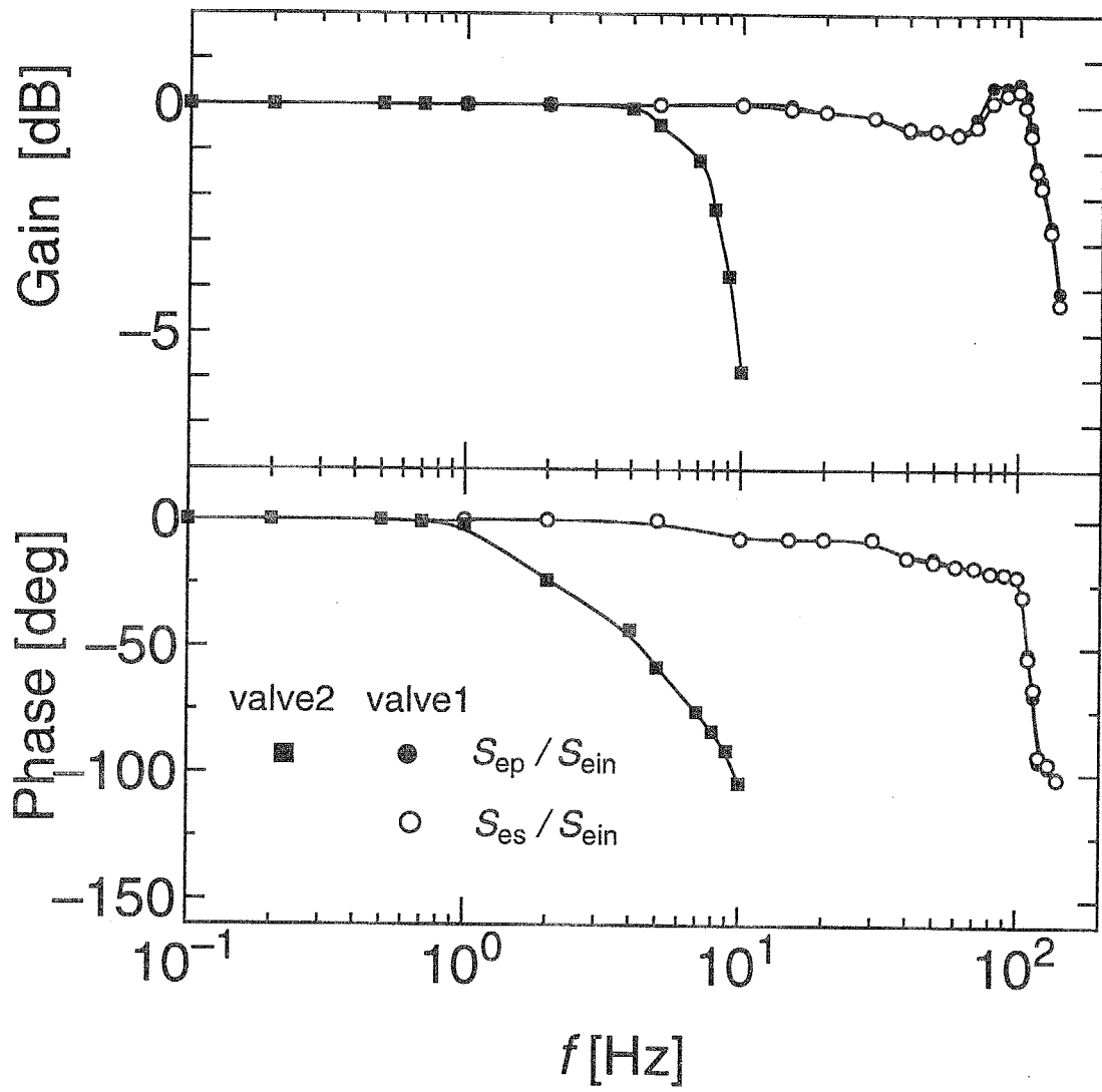
Fig.6.9 Bode diagram of the tested valve (3port)
