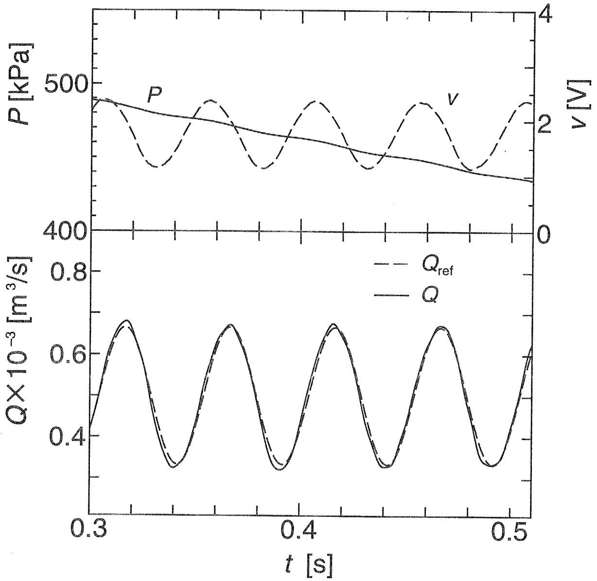
Fig.7.6 Unsteady flow rate measurement ( K_p = 2.0[\text{V} \cdot \text{s}/\text{Pa}] , T_i = 20[\text{s}] , f = 20[\text{Hz}] )
