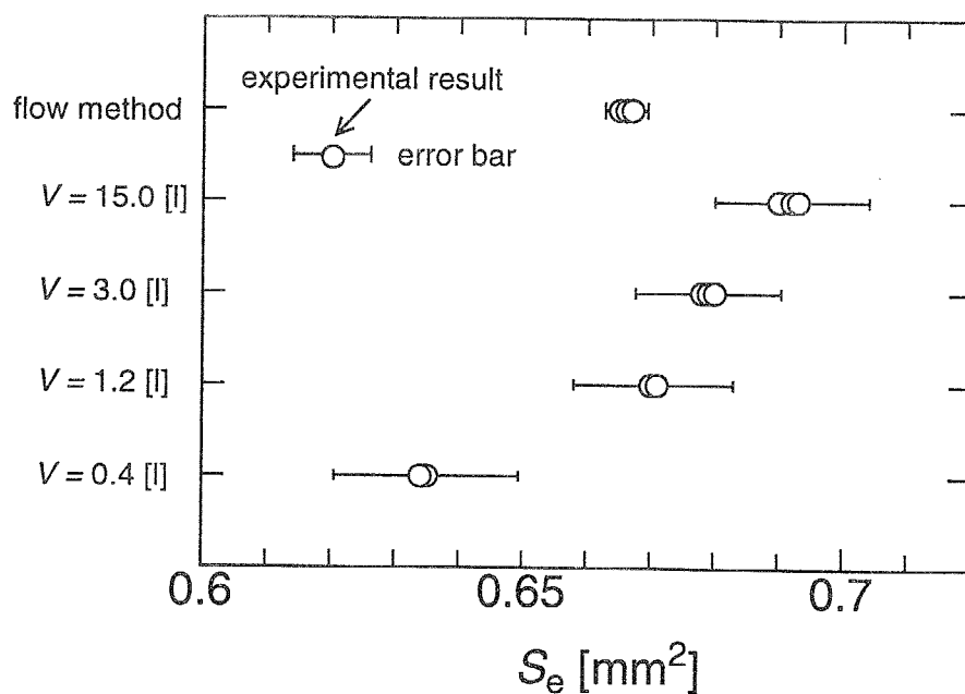
Fig.5.5 The effect of the tank volume
