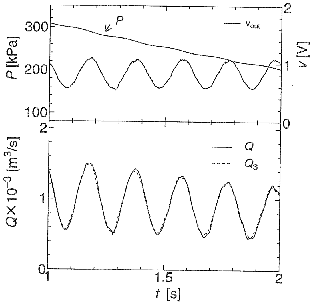
Fig.4.13 Unsteady flow rate measurement with the isothermal chamber( f=5 [Hz])
