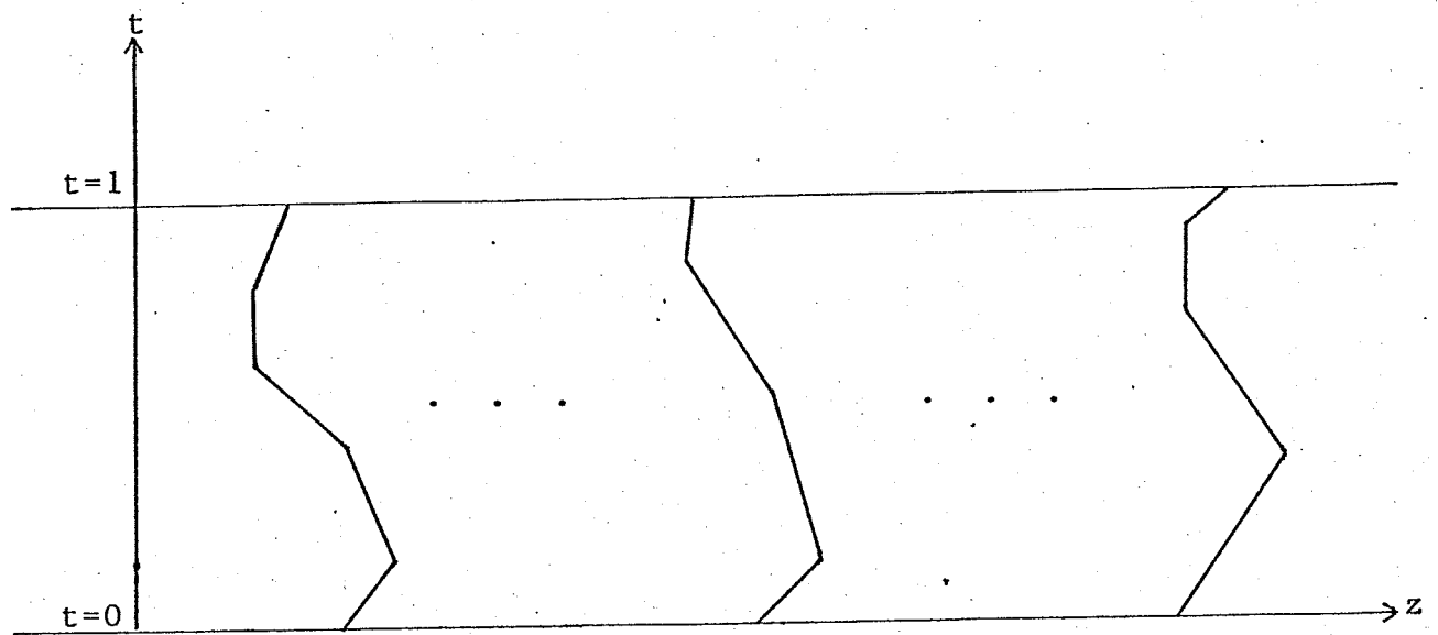
Fig.2. . . Solution set \Delta^* .
