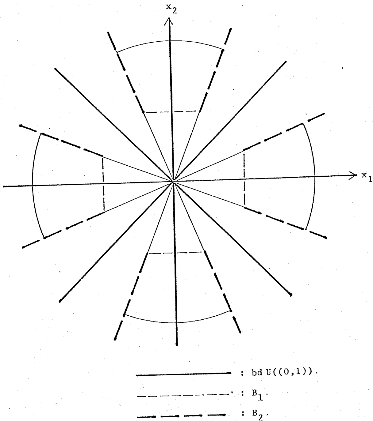
Fig.5. \text{bd } U((0,1)) , B_1 and B_2 ( d=4 ).
