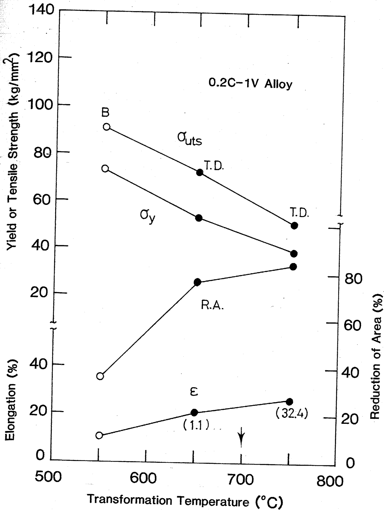
re 3-5 Tensile properties of isothermally transformed Alloy 1 following an austenitization at 1000°C.
