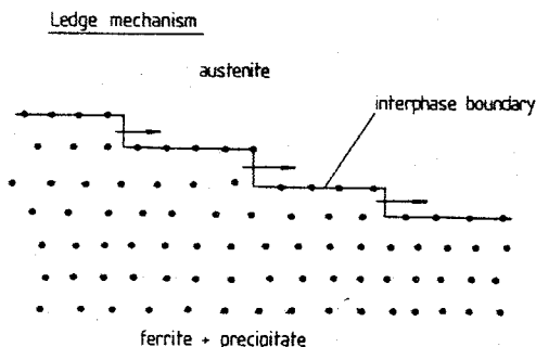
Fig. 5-8 Ledge mechanism in the growth of ferrite associated with interphase precipitation. (7,47)
