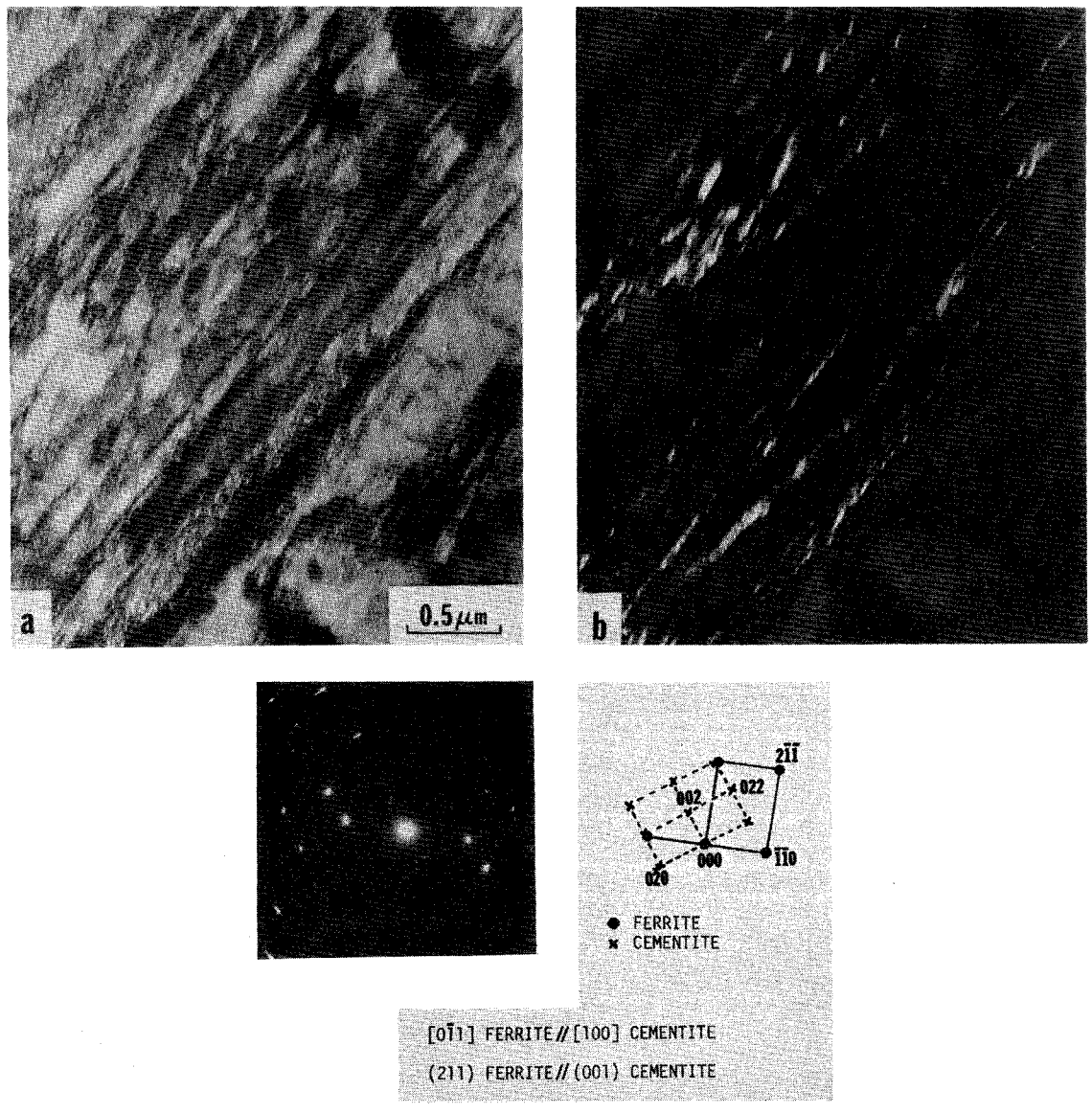
Figure 2-11 Transmission electron micrograph of Alloy 3 ausaged at 700°C for 1 hour showing a typical auto-tempered martensitic microstructure.
