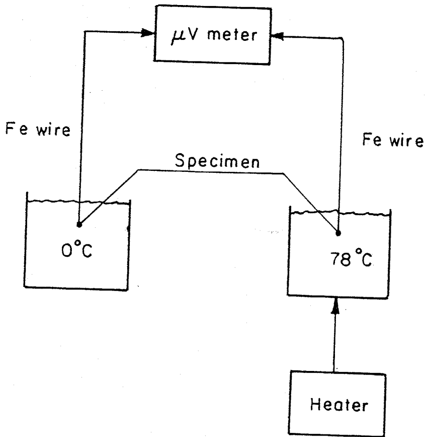
Fig. 2-2 Schematic representation of thermo-electric potential measurement apparatus.
