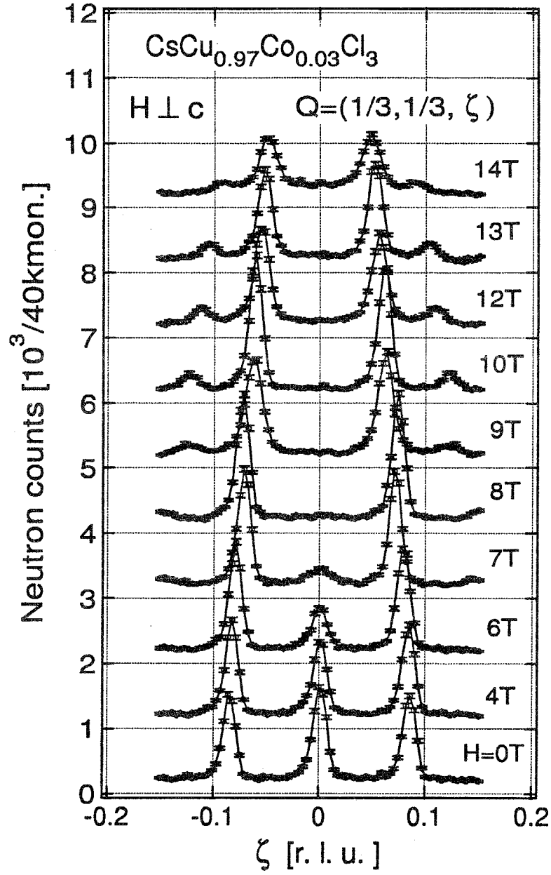
Figure 3.24: The scans along \mathbf{Q} = (1/3, 1/3, \zeta) in the vicinity of \zeta = 0 at various magnetic field applied perpendicular to the c -axis. The measurements were performed at T = 2\text{ K} .
