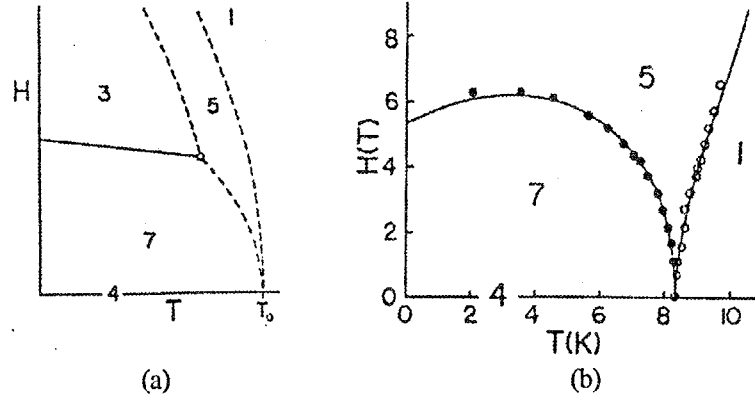
Figure 2.3: (a) Schematic phase diagram for H \perp c and A_z < 0, B_2 > 0, B_4 > 0 . Solid line and the open circle indicates the first-order spin-flop transition and the multicritical point, respectively. Dashed lines indicate the second order transition. (b) Phase diagram of \text{CsMnBr}_3 . Closed and open circles are the experimental data measured by Gaulin et al. [36] Solid lines are the fitting result by Plumer et al. The definitions of the numbers are described in the text. (quoted from ref. [21, 19])
