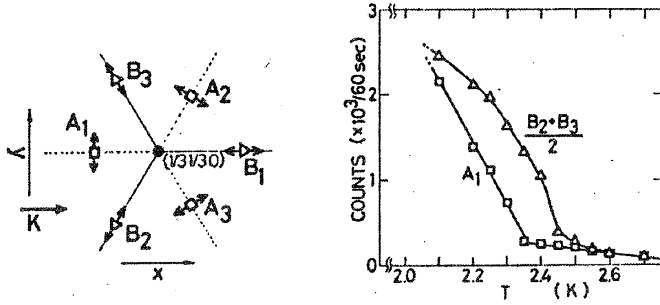
Figure 4.2: The temperature dependences of the scattering intensity of the A_1 peak and the mean value of the intensities at the B_2 and B_3 peaks, where A_1 , B_2 and B_3 are the reciprocal lattice points which are shown in left figure. (quoted from ref. [110])
