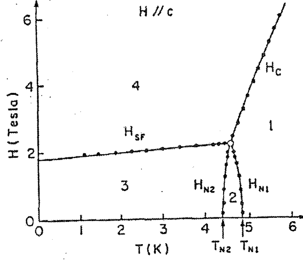
Figure 2.2: The phase diagram of \text{CsNiCl}_3 . Solid circles indicate the experimental data measured by Johnson et al. [15]. Solid lines are the fitting result by Plumer et al. (quoted from ref. [18])
