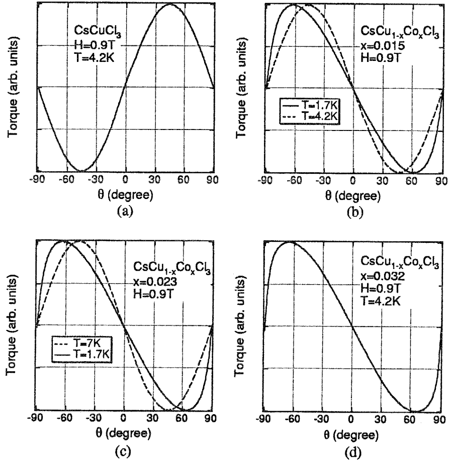
Figure 3.14: Torque curves for (a) \text{CsCuCl}_3 and \text{CsCu}_{1-x}\text{Co}_x\text{Cl}_3 with (b) x = 0.015 , (c) 0.023 and (d) 0.032 . The external field of 0.9\text{ T} is rotated in the ac -plane. In (b) and (c), solid and dashed lines denote the torque curves in phase II and I, respectively.
