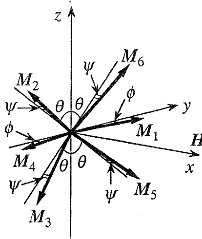
Figure 2.4: The spin configuration in the spin-flop phase of the Heisenberg TAF with weak planar anisotropy. (quoted from ref. [17].)
