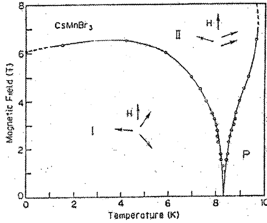
Figure 2.8: The phase diagram of CsMnBr 3 in a magnetic field applied in the c -plane. Transition points were determined by the magnetization measurements.
