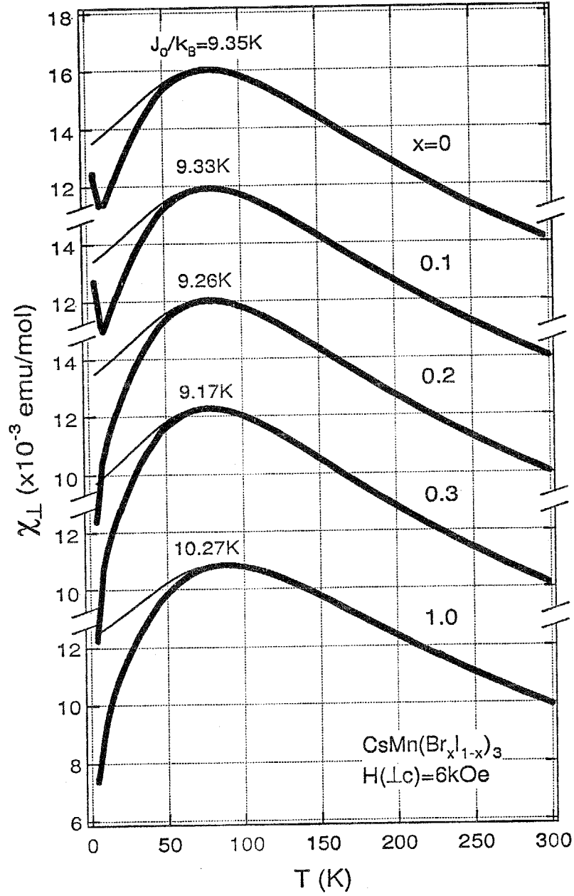
Figure 2.13: The temperature dependences of the perpendicular susceptibilities \chi_{\perp} for the \text{CsMn}(\text{Br}_x\text{I}_{1-x})_3 system measured at H = 6 \text{ kOe} . The thick lines show the experimental results and thin solid lines represent fits of Fisher's theory to our data for T > 90 \text{ K} .
