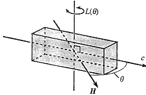
Figure 2.12: The experimental geometry of the torque measurements.
