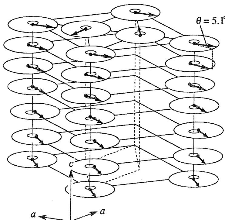
Figure 3.3: The magnetic structure of CsCuCl 3 in the ground state. Solid circles at the root of each spins indicate the displacement from the c -axis of Cu 2+ ion. The angle \theta \simeq 5.1^\circ denotes the pitch of the helical structure along the c -axis per Cu-site.
