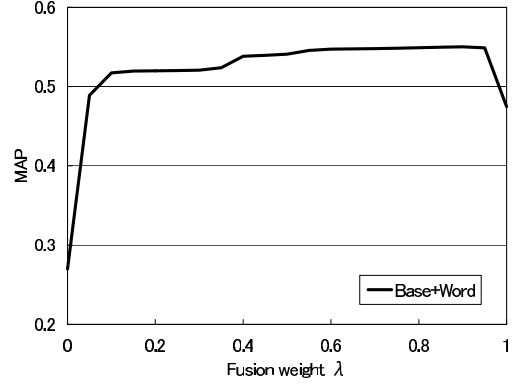
Figure 2: Fusion results of phone- and word-based detection
